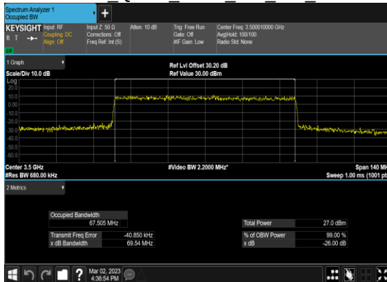
N77(70M)_CP-OFDM_QPSK Outer Full Mid CH
