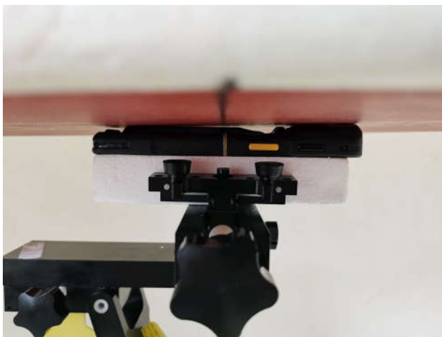
Back_ Extended, Test Separation 0 mm
