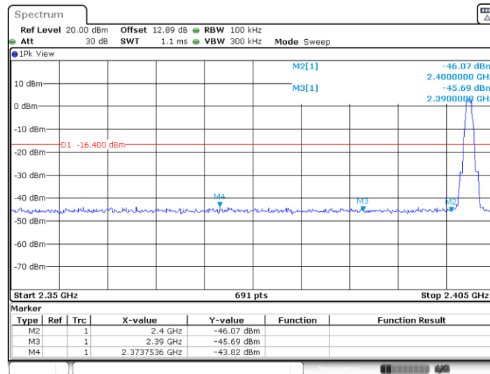
BLE_1M_Ant7_Low_2402
