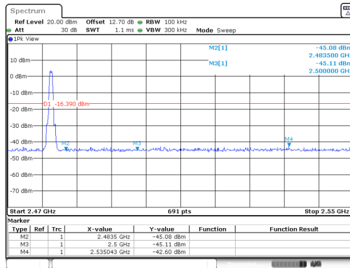
BLE_1M_Ant7_High_2480
