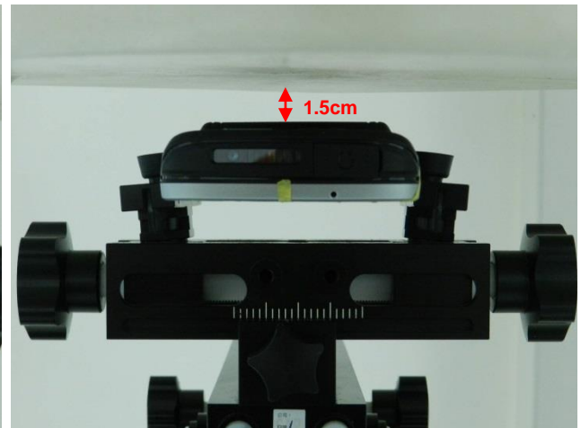
Back With Battery 2, Test Separation 1.5 cm
