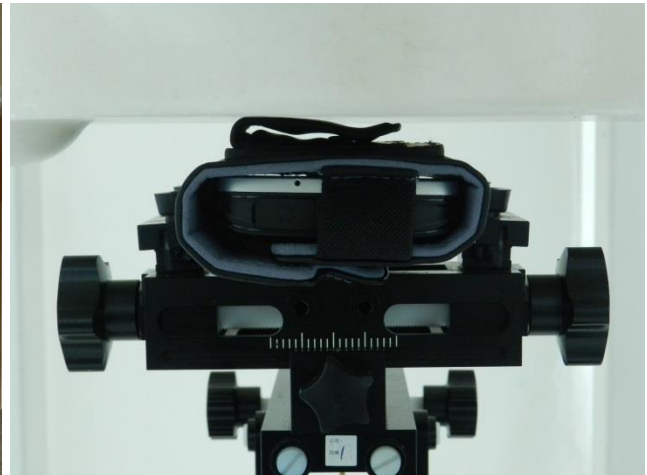
Back With Battery 1 and Holster, Test Separation 0 cm
