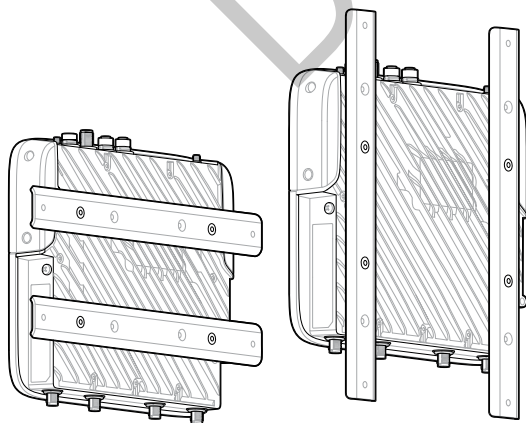
Figure 8 Bracket Orientations
