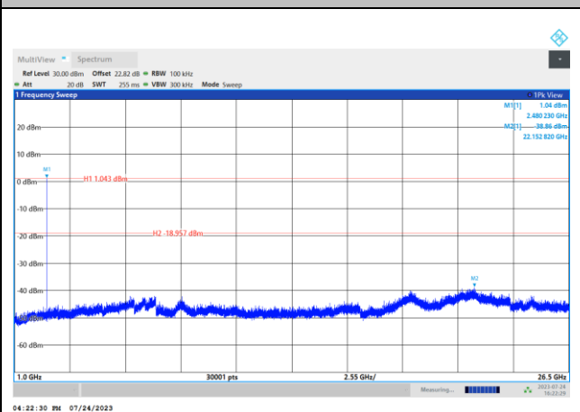
CSE Plot on Ch 78 between 1 GHz ~ 26.5 GHz
