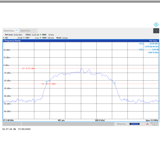
20 dB Bandwidth Plot on Channel 78
