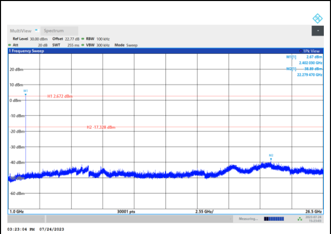
CSE Plot on Ch 00 between 1 GHz ~ 26.5 GHz
