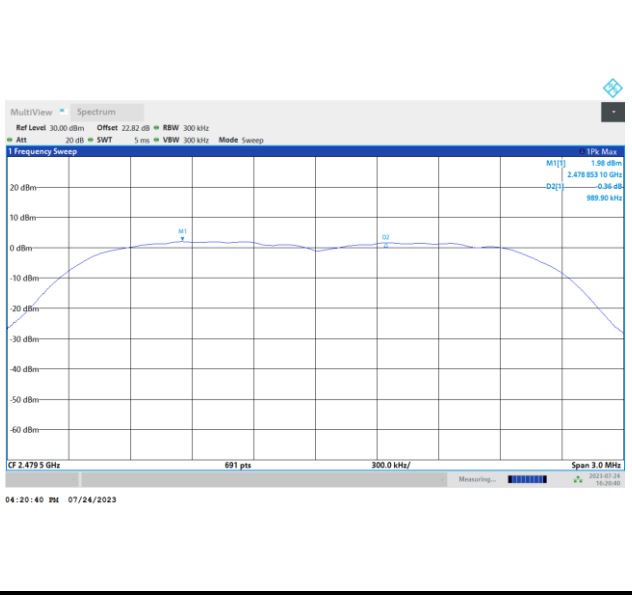
Channel Separation Plot on Channel 77 - 78
