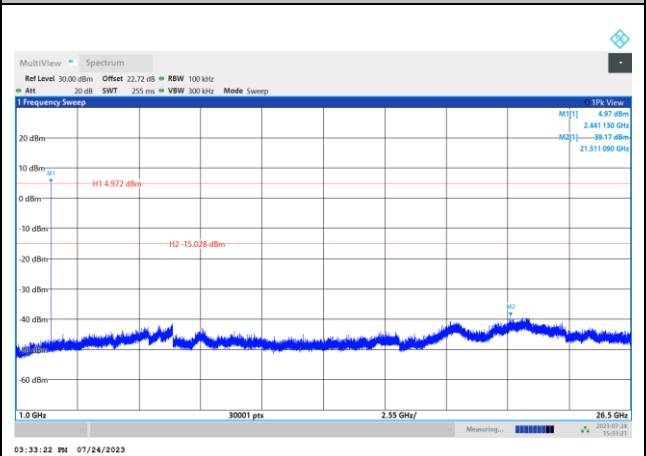
CSE Plot on Ch 39 between 1 GHz ~ 26.5 GHz
