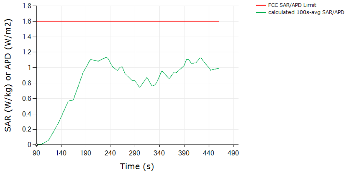
SAR (or APD) (Test Sequence 2) Tech: LTE, Band 2
