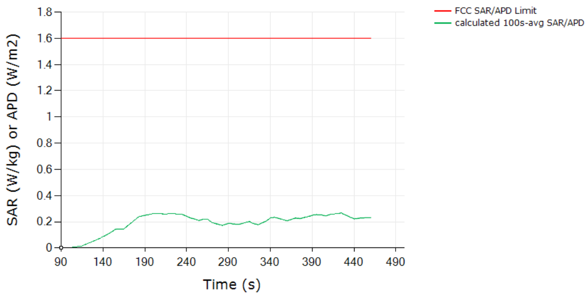
SAR (or APD) (Test Sequence 2) Tech: WCDMA, Band 5
