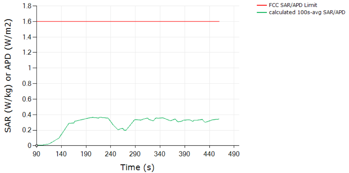
SAR (or APD) (Test Sequence 2) Tech: WCDMA, Band 4
