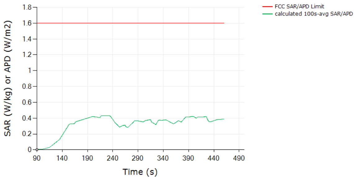
SAR (or APD) (Test Sequence 2) Tech: LTE, Band 66
