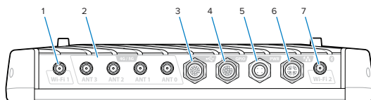
Figure 1 FXR90 Top Panel Connections
