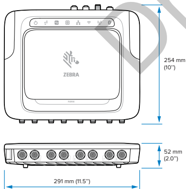
Figure 4 FXR90 Mechanical Dimensions
