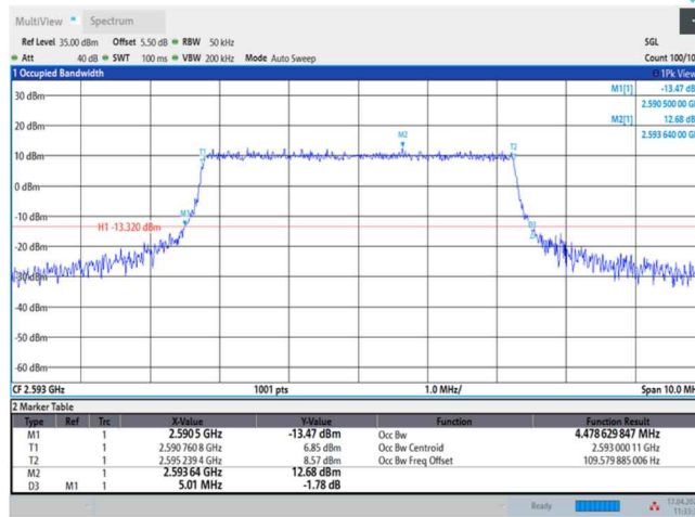
Band41-5MHz-QPSK-40620-25RB#0
