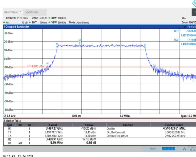
Band42-5MHz-QPSK-42590-25RB#0
