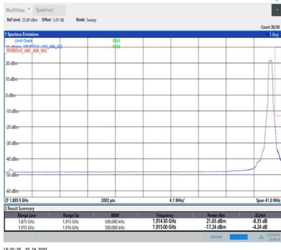
1-N25--15-40-H-2-DFT-PI2BPSK-Edge_1RB_Right-1@215-Ant0-seegraph-PASS-see graph
