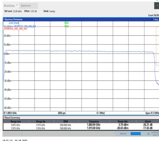
1-N25--15-40-H-3-DFT-PI2BPSK-Outer_Full-216@0-Ant0-seegraph-PASS-see graph
