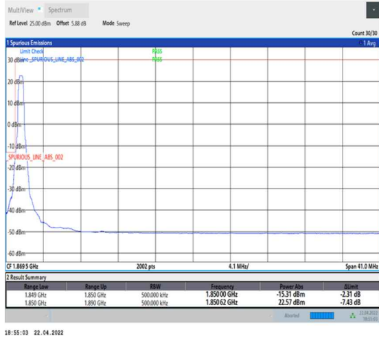
1-N25--15-40-L-1-DFT-PI2BPSK-Edge_1RB_Left-1@0-Ant0-seegraph-PASS-see graph
