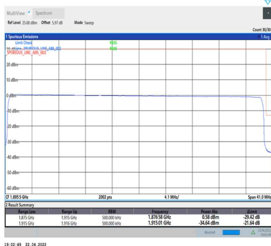
1-N25--15-40-H-6-CP-QPSK-Outer_Full-216@0-Ant0-seegraph-PASS-see graph
