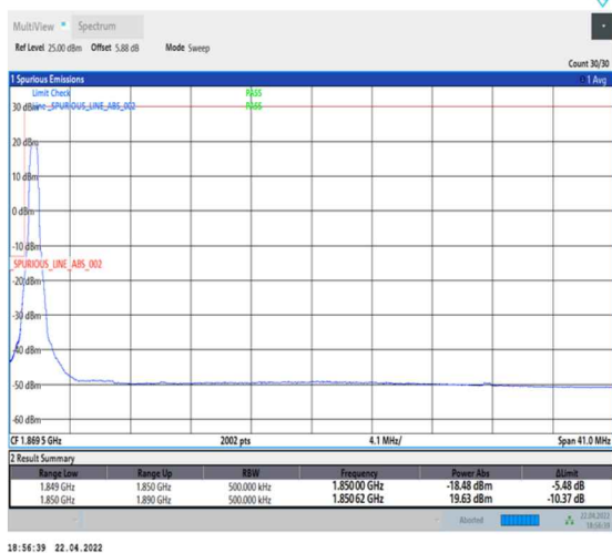
1-N25--15-40-L-4-CP-QPSK-Edge_1RB_Left-1@0-Ant0-seegraph-PASS-see graph
