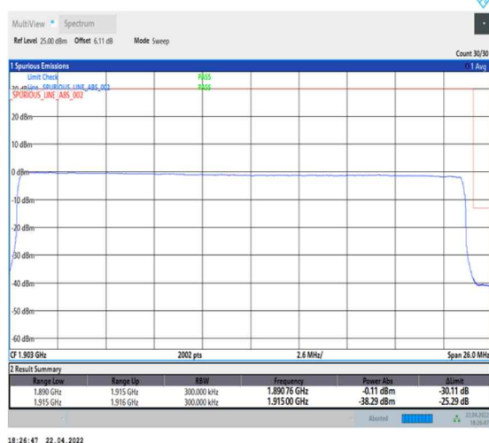
1-N25--15-25-H-6-CP-QPSK-Outer_Full-133@0-Ant0-seegraph-PASS-see graph
