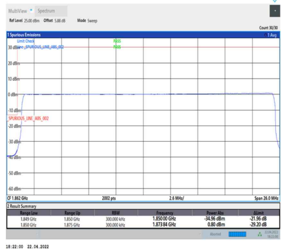
1-N25--15-25-L-6-CP-QPSK-Outer_Full-133@0-Ant0-seegraph-PASS-see graph
