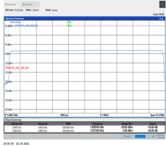
1-N25--15-40-L-3-DFT-PI2BPSK-Outer_Full-216@0-Ant0-seegraph-PASS-see graph
