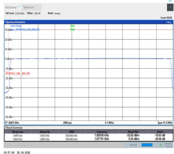
1-N25--15-40-L-6-CP-QPSK-Outer_Full-216@0-Ant0-seegraph-PASS-see graph
