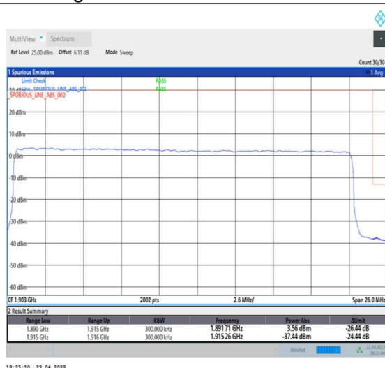
1-N25--15-25-H-3-DFT-PI2BPSK-Outer_Full-128@0-Ant0-seegraph-PASS-see graph
