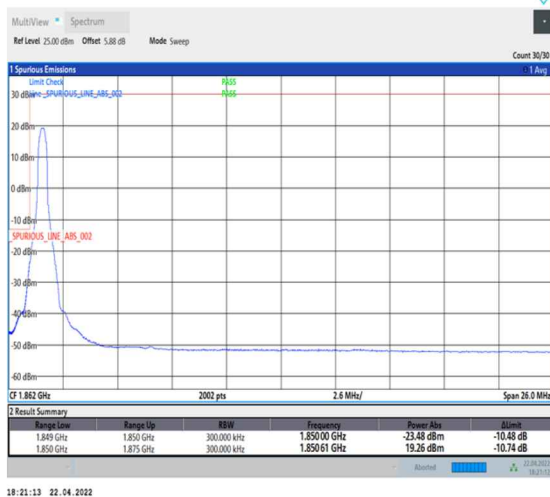
1-N25--15-25-L-4-CP-QPSK-Edge_1RB_Left-1@0-Ant0-seegraph-PASS-see graph
