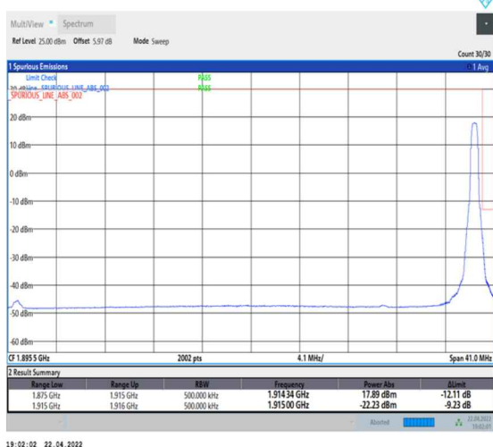
1-N25--15-40-H-5-CP-QPSK-Edge_1RB_Right-1@215-Ant0-seegraph-PASS-see graph
