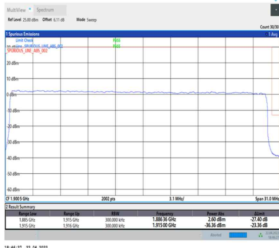
1-N25--15-30-H-3-DFT-PI2BPSK-Outer_Full-160@0-Ant0-seegraph-PASS-see graph
