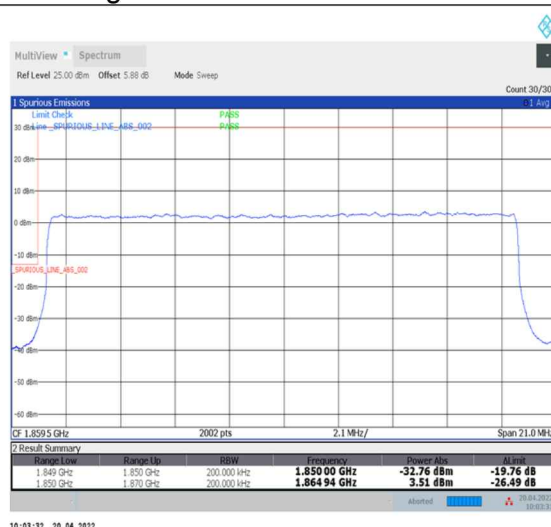
1-N25--15-20-L-3-DFT-PI2BPSK-Outer_Full-100@0-Ant0-seegraph-PASS-see graph
