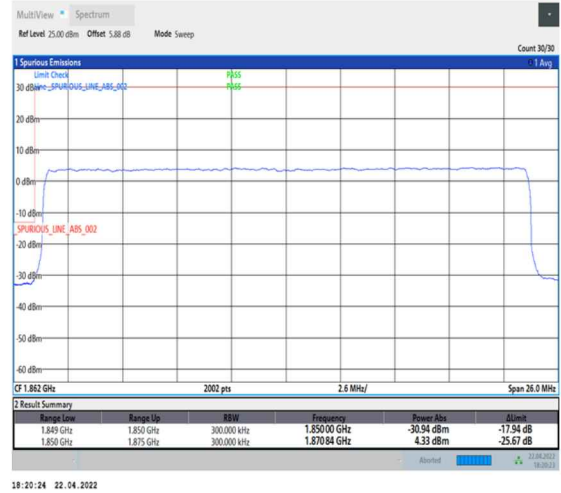
1-N25--15-25-L-3-DFT-PI2BPSK-Outer_Full-128@0-Ant0-seegraph-PASS-see graph
