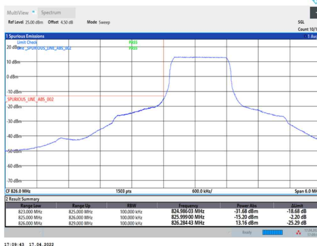
Band5-1.4MHz-QPSK-20427-6RB#0
