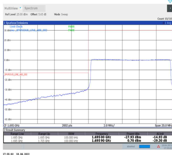
1-N70--15-10-L-6-CP-QPSK-Outer_Full-52@0-Ant2-seegraph-PASS-see graph
