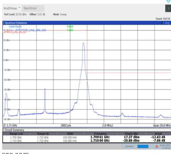
1-N70--15-10-H-5-CP-QPSK-Edge_1RB_Right-1@51-Ant2-seegraph-PASS-see graph
