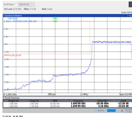
1-N70--15-5-L-3-DFT-PI2BPSK-Outer_Full-25@0-Ant2-seegraph-PASS-see graph
