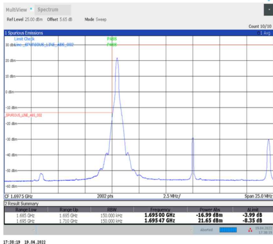
1-N70--15-15-L-1-DFT-PI2BPSK-Edge_1RB_Left-1@0-Ant2-seegraph-PASS-see graph
