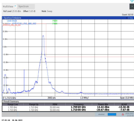
1-N70--15-5-H-5-CP-QPSK-Edge_1RB_Right-1@24-Ant2-seegraph-PASS-see graph
