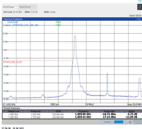
1-N70--15-10-L-4-CP-QPSK-Edge_1RB_Left-1@0-Ant2-seegraph-PASS-see graph
