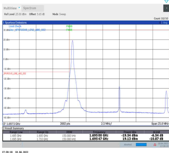
1-N70--15-15-L-4-CP-QPSK-Edge_1RB_Left-1@0-Ant2-seegraph-PASS-see graph
