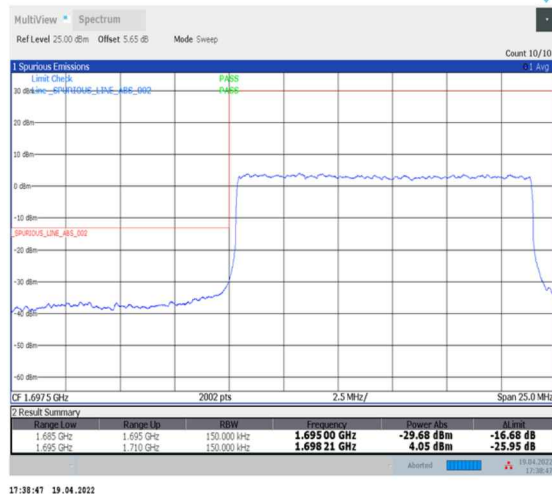
1-N70--15-15-L-3-DFT-PI2BPSK-Outer_Full-75@0-Ant2-seegraph-PASS-see graph
