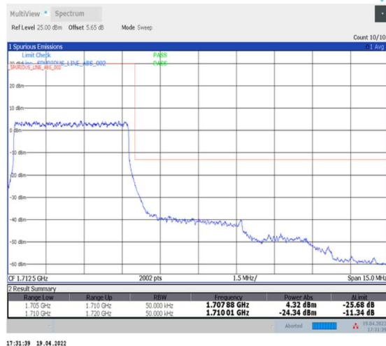
1-N70--15-5-H-3-DFT-PI2BPSK-Outer_Full-25@0-Ant2-seegraph-PASS-see graph
