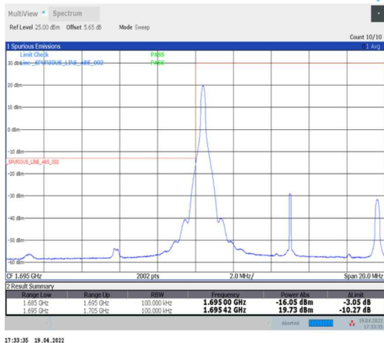
1-N70--15-10-L-1-DFT-PI2BPSK-Edge_1RB_Left-1@0-Ant2-seegraph-PASS-see graph
