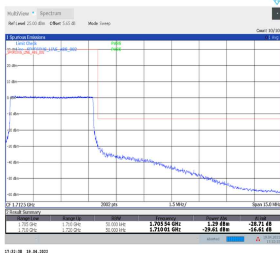
1-N70--15-5-H-6-CP-QPSK-Outer_Full-25@0-Ant2-seegraph-PASS-see graph
