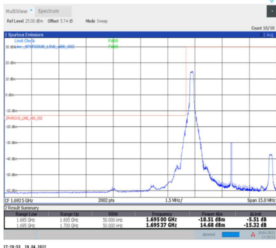
1-N70--15-5-L-4-CP-QPSK-Edge_1RB_Left-1@0-Ant2-seegraph-PASS-see graph
