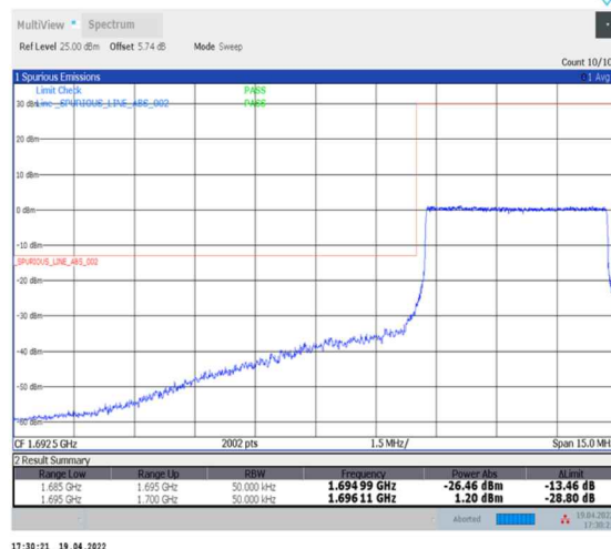
1-N70--15-5-L-6-CP-QPSK-Outer_Full-25@0-Ant2-seegraph-PASS-see graph
