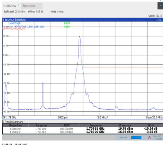
1-N70--15-10-H-2-DFT-PI2BPSK-Edge_1RB_Right-1@51-Ant2-seegraph-PASS-see graph
