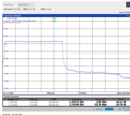
1-N70--15-10-H-3-DFT-PI2BPSK-Outer_Full-50@0-Ant2-seegraph-PASS-see graph
