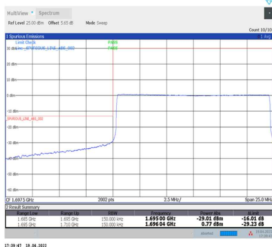
1-N70--15-15-L-6-CP-QPSK-Outer_Full-79@0-Ant2-seegraph-PASS-see graph
