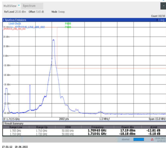
1-N70--15-5-H-2-DFT-PI2BPSK-Edge_1RB_Right-1@24-Ant2-seegraph-PASS-see graph
