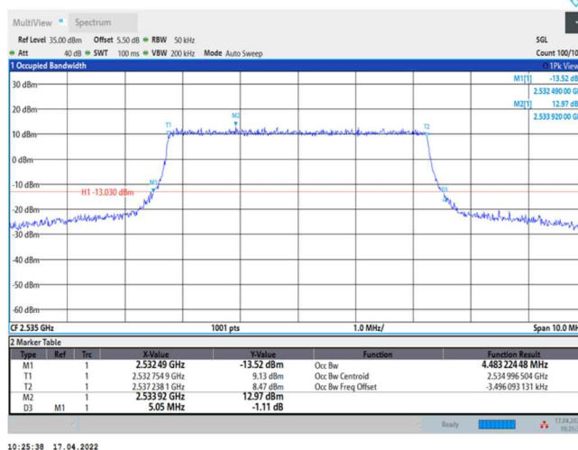
Band7-5MHz-QPSK-21100-25RB#0
