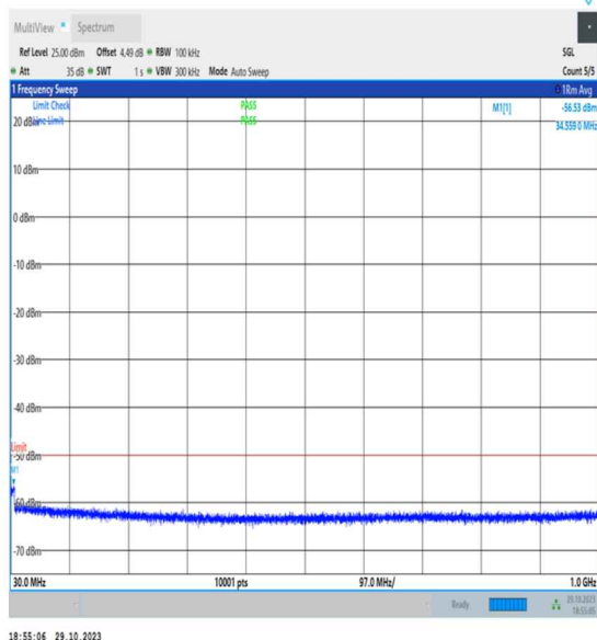
NTVN_N48_PC3_30_30_L_TID1_NS_01_30_1000_#1
