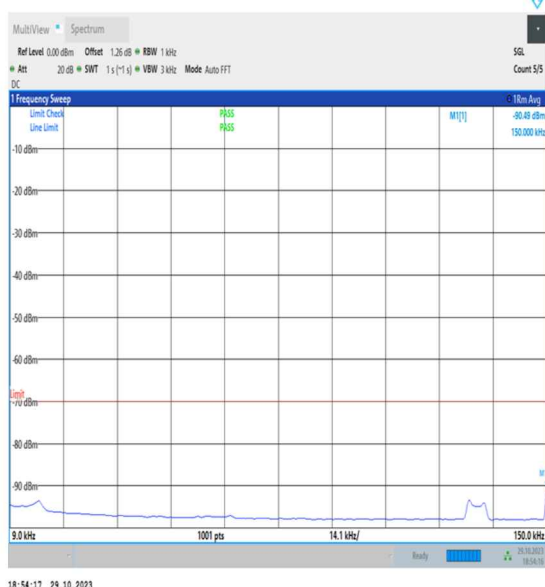
NTVN_N48_PC3_30_30_L_TID1_NS_01_0.009_0.15_#1
