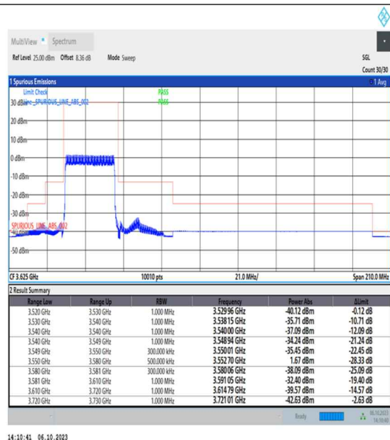
NTNV_N48_PC3_30_30_L_TID3_RID1#1
