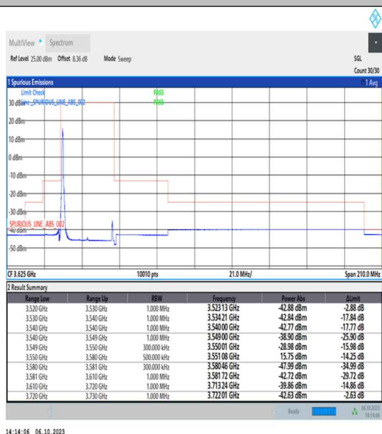
NTNV_N48_PC3_30_30_L_TID4_RID1#1
