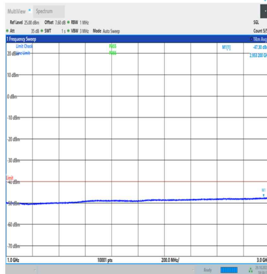
NTNV_N48_PC3_30_30_H_TID1_NS_01_1000_3000_#1
