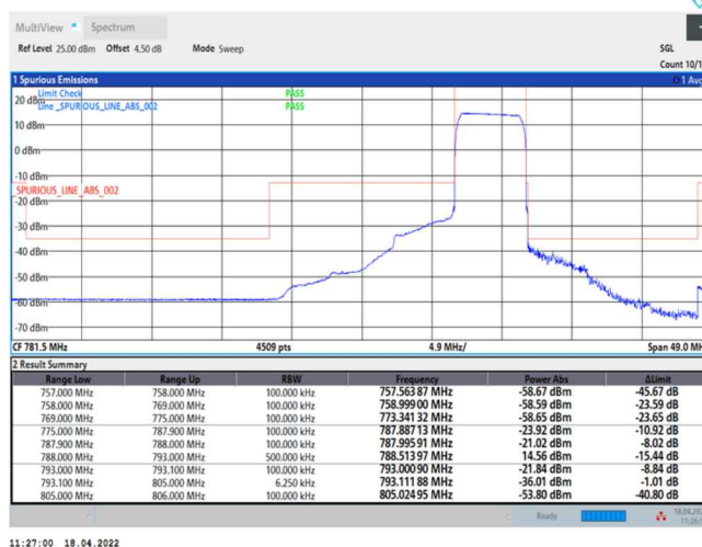
Band14-5MHz-QPSK-23305-25RB#0
