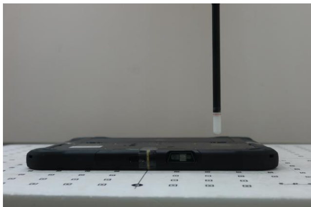
Bottom Face at 14 mm
