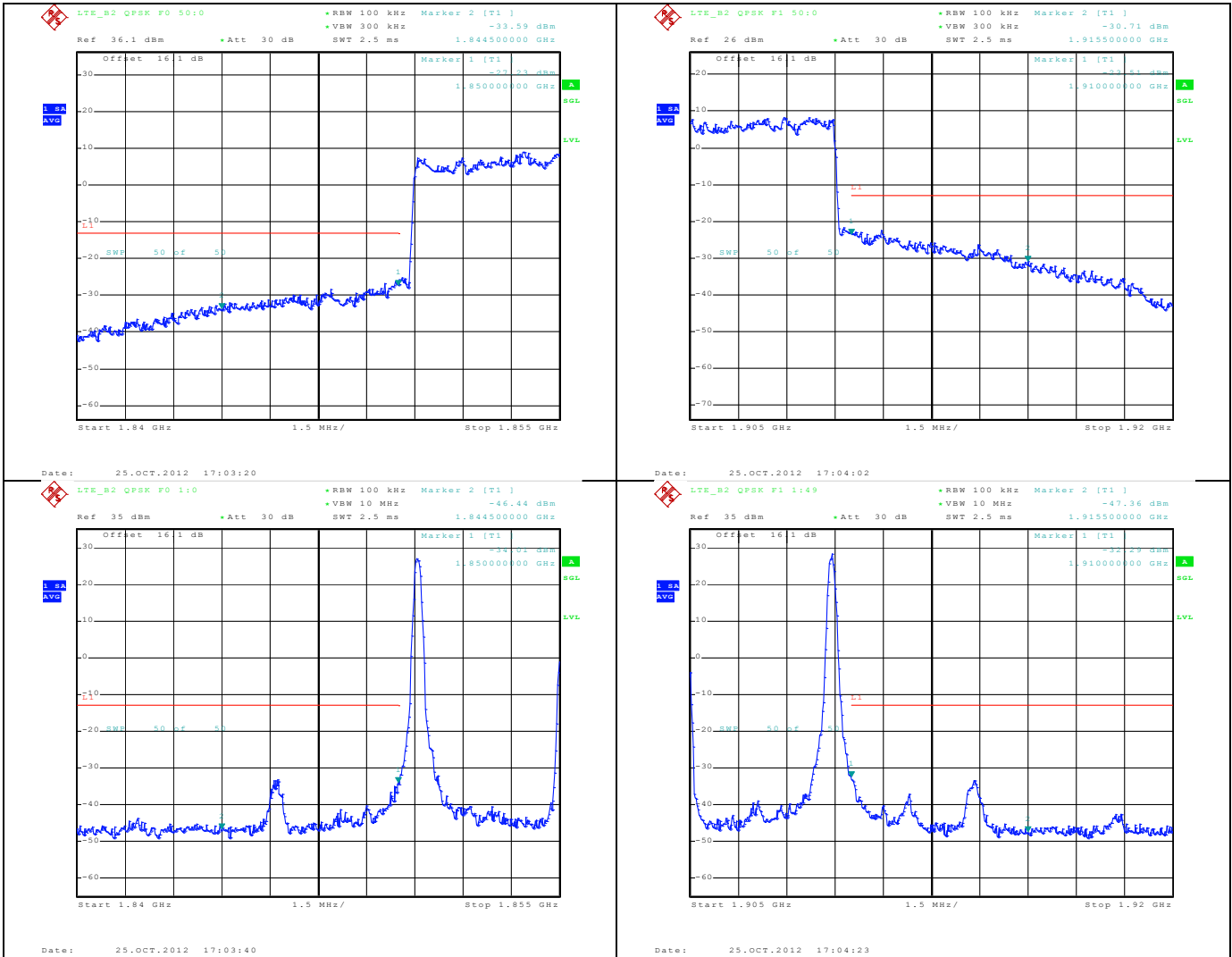
9.2.1.3 LTE; Band2, 15 MHz BW, QPSK
