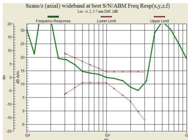
Fig. 9.12 WCDMA Band V Ch4233 – Battery 1
