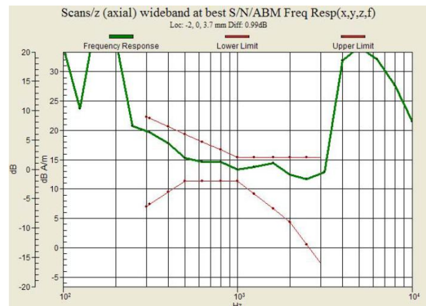
Fig. 9.6 GSM1900 Ch661 – Battery 2
