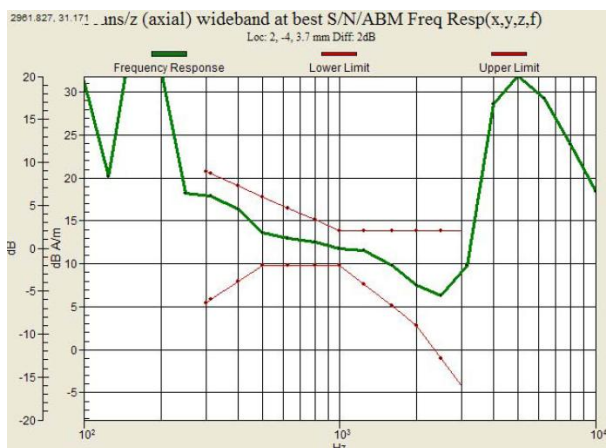
Fig. 9.9 WCDMA Band V Ch4182 – Battery 1
