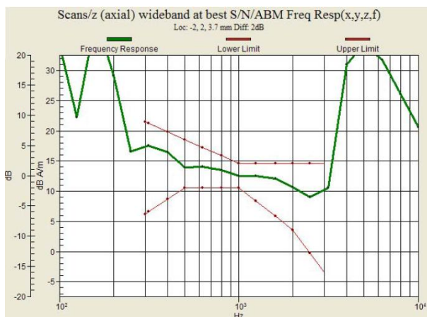
Fig. 9.21 CDMA2000 BC0 Ch600 – Battery 1
