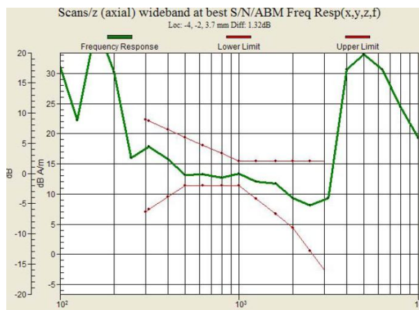
Fig. 9.18 CDMA2000 BC0 Ch384 – Battery 2
