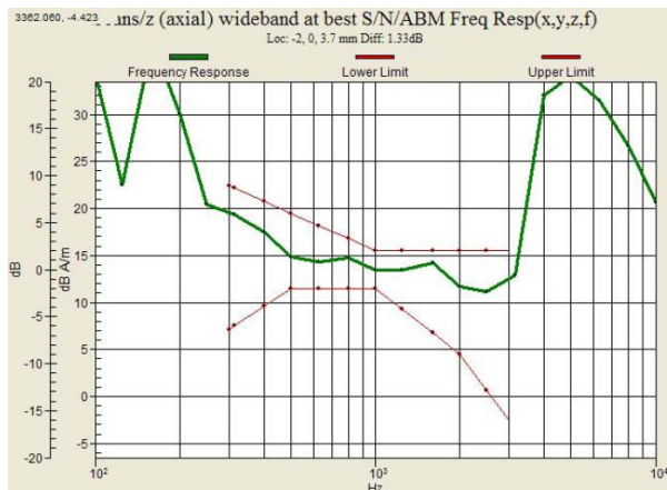
Fig. 9.3 GSM850 Ch128 – Battery 1
