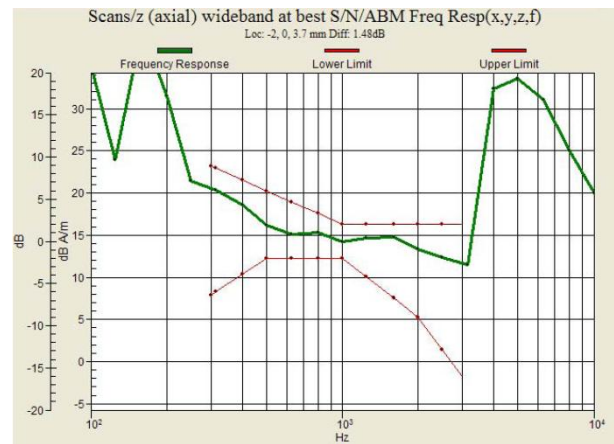
Fig. 9.2 GSM850 Ch189 – Battery 2
