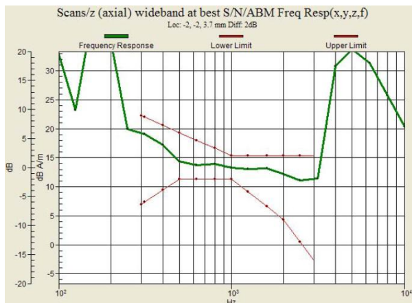
Fig. 9.5 GSM1900 Ch661 – Battery 1
