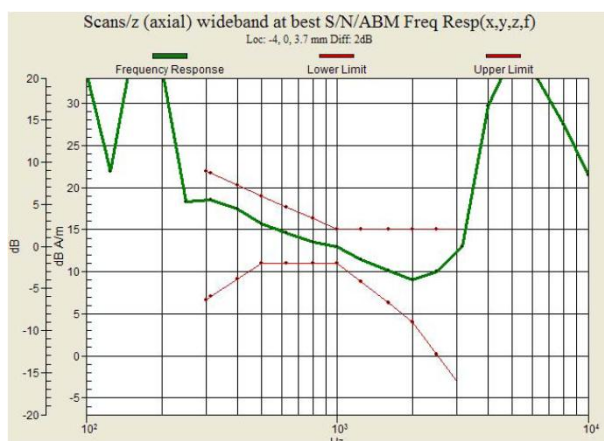
Fig. 9.19 CDMA2000 BC0 Ch1013 – Battery 1
