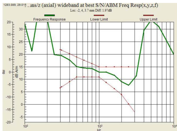
Fig. 9.11 WCDMA Band V Ch4132 – Battery 1
