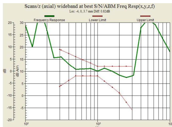
Fig. 9.20 CDMA2000 BC0 Ch777 – Battery 1
