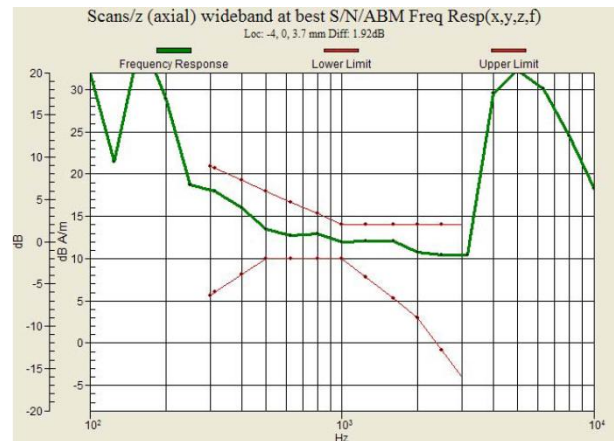
Fig. 9.4 GSM850 Ch251 – Battery 1
