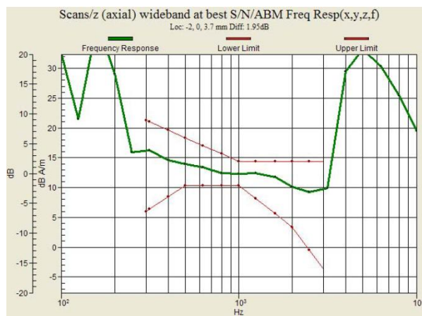
Fig. 9.22 CDMA2000 BC0 Ch600 – Battery 2
