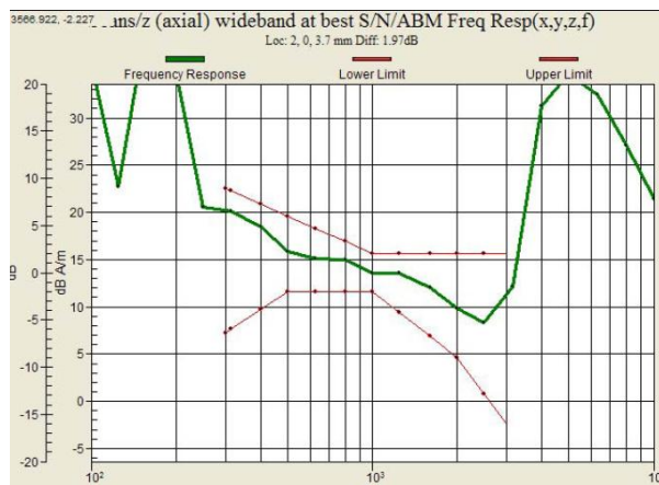
Fig. 9.16 WCDMA Band II Ch9538 – Battery 2
