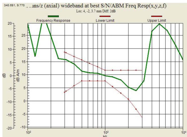
Fig. 9.15 WCDMA Band II Ch9262 – Battery 2
