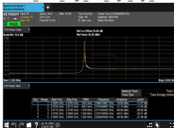
N7(20M)_DFT-s- OFDM_BPSK_Edge_1RB_Right_High_CH
