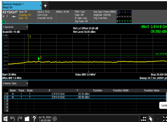
N7(40M)_DFT-s- OFDM_QPSK_Edge_1RB_Left_Mid_CH
