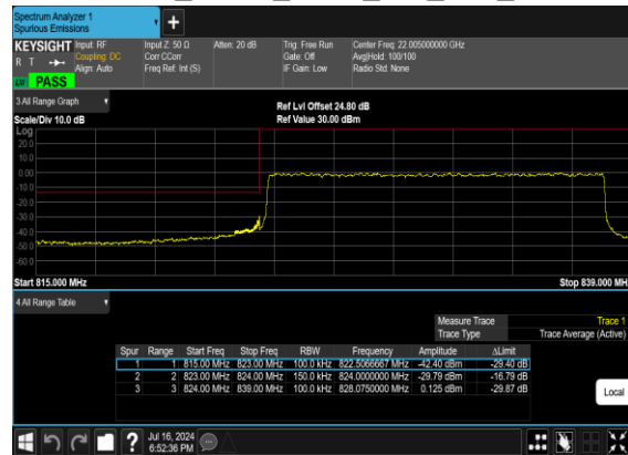
N26(15M)_DFT-s- OFDM_QPSK_Outer_Full_Low_CH
