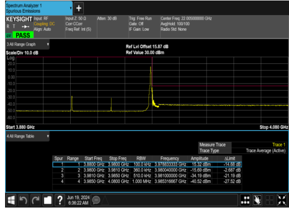
B2_N77(60M)_DFT-s-OFDM_QPSK_Edge_1RB_Right_High_CH
