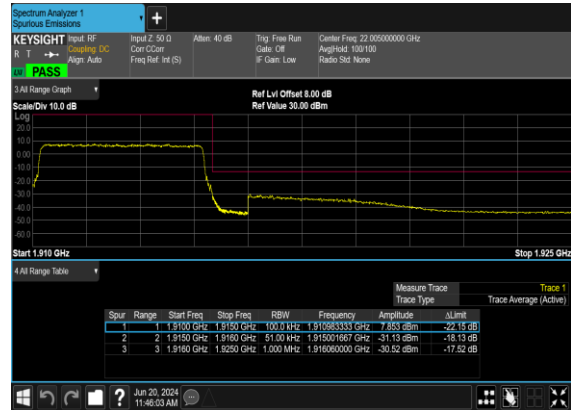
B12_N25(5M)_DFT-s- OFDM_QPSK_Outer_Full_High_CH
