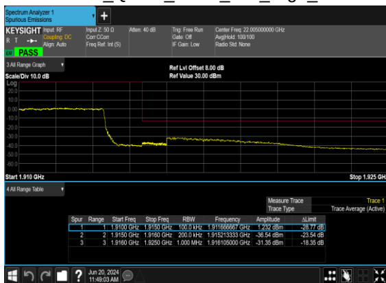
B12_N25(20M)_DFT-s- OFDM_QPSK_Outer_Full_High_CH
