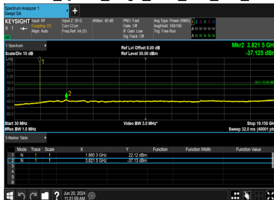
B12_N25(5M)_DFT-s-OFDM_QPSK_Edge_1RB_Left_Mid_CH
