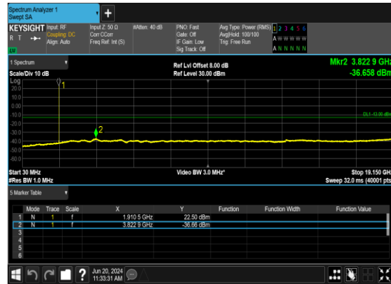
B12_N25(5M)_DFT-s-OFDM_QPSK_Edge_1RB_Left_High_CH
