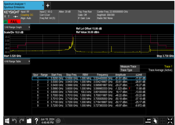
B2_N77(100M)_DFT-s- OFDM_QPSK_Edge_1RB_Left_High_CH
