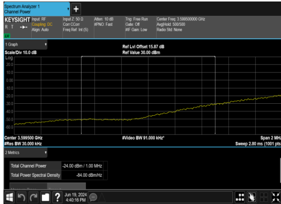
B2_N77(100M)_DFT-s- OFDM_BPSK_Edge_1RB_Left_High_CH_CHP_PASS
