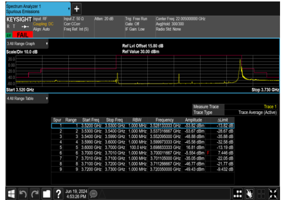
B2_N77(100M)_DFT-s- OFDM_BPSK_Edge_1RB_Right_High_CH
