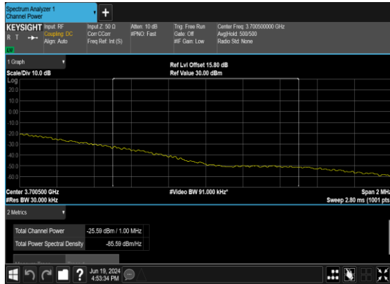
B2_N77(100M)_DFT-s- OFDM_BPSK_Edge_1RB_Right_High_CH_CHP_PASS
