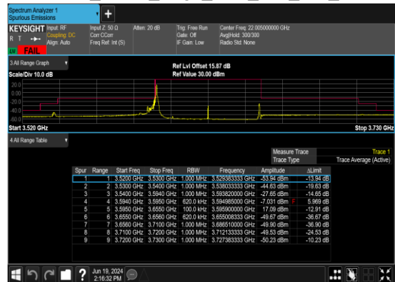
B2_N77(60M)_DFT-s-OFDM_BPSK_Edge_1RB_Left_Mid_CH
