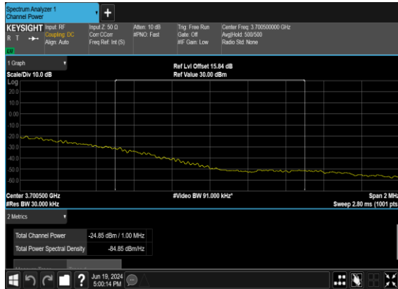
B2_N77(100M)_DFT-s- OFDM_QPSK_Edge_1RB_Right_High_CH_CHP_PASS
