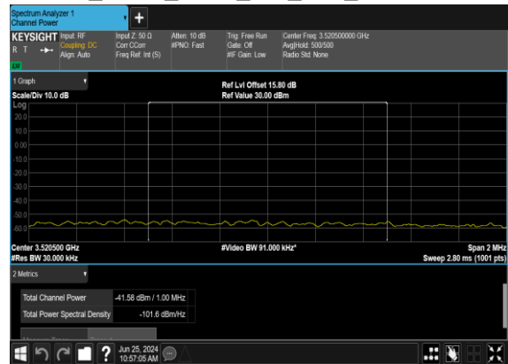
B2_N77(60M)_DFT-s-OFDM_BPSK_Outer_Full_Low_CH_CHP_PASS
