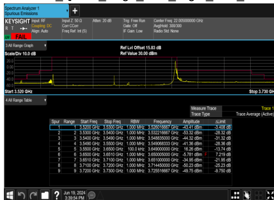
B2_N77(100M)_DFT-s- OFDM_QPSK_Edge_1RB_Right_Low_CH
