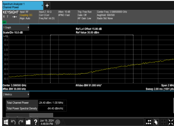
B2_N77(100M)_DFT-s- OFDM_QPSK_Edge_1RB_Left_High_CH_CHP_PASS
