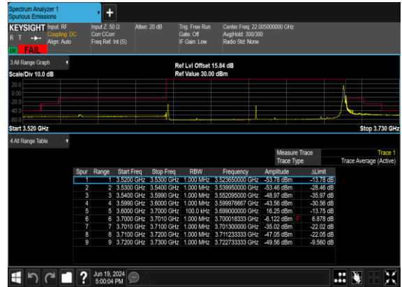
B2_N77(100M)_DFT-s- OFDM_QPSK_Edge_1RB_Right_High_CH
