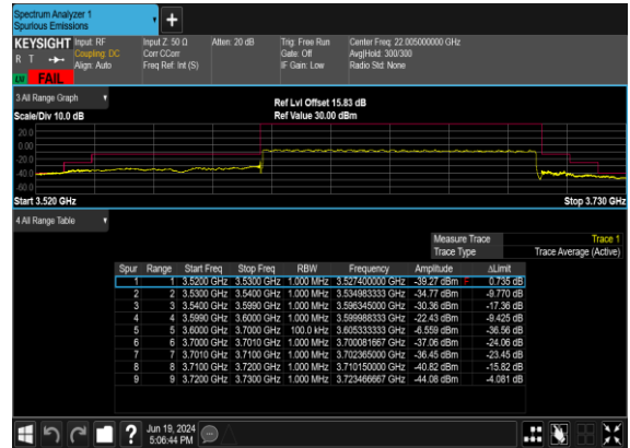
B2_N77(100M)_DFT-s- OFDM_BPSK_Outer_Full_High_CH
