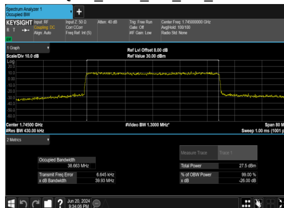
B2_N66(40M)_CP-OFDM_16 QAM_Outer_Full_Mid_CH
