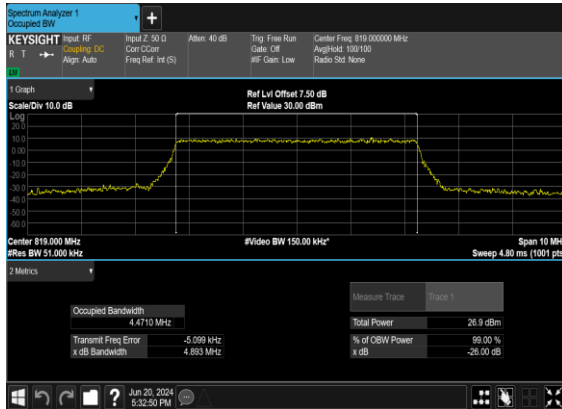
N26(5M)_CP-OFDM_QPSK_Outer_Full_Mid_CH
