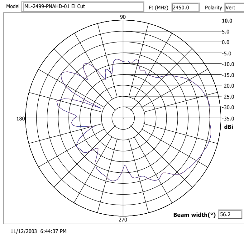
Elevation Pattern
