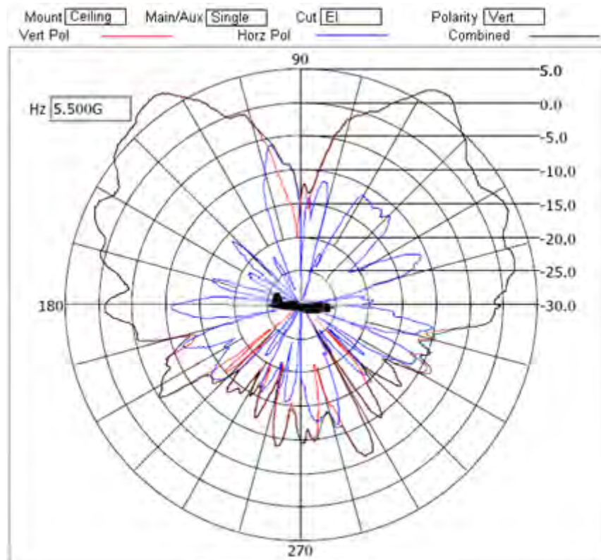
Elevation Pattern
