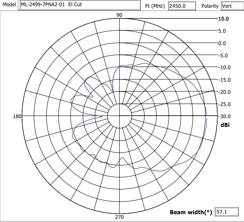
Elevation Cut
