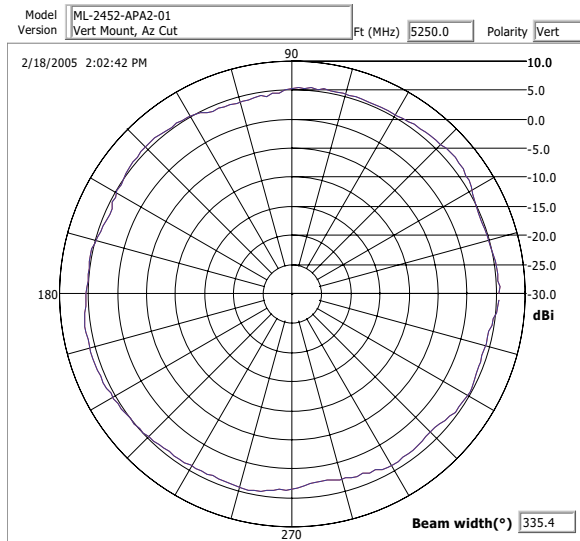
Azimuth Pattern
