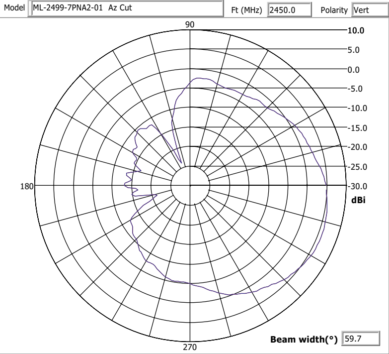
Azimuth Cut
