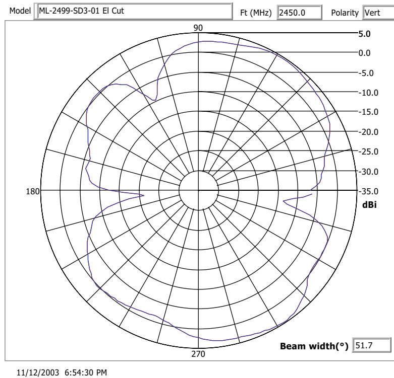
Elevation Pattern
