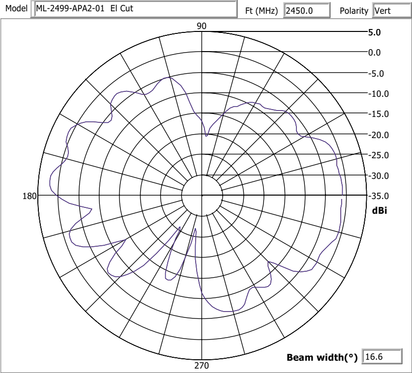
Elevation Pattern
