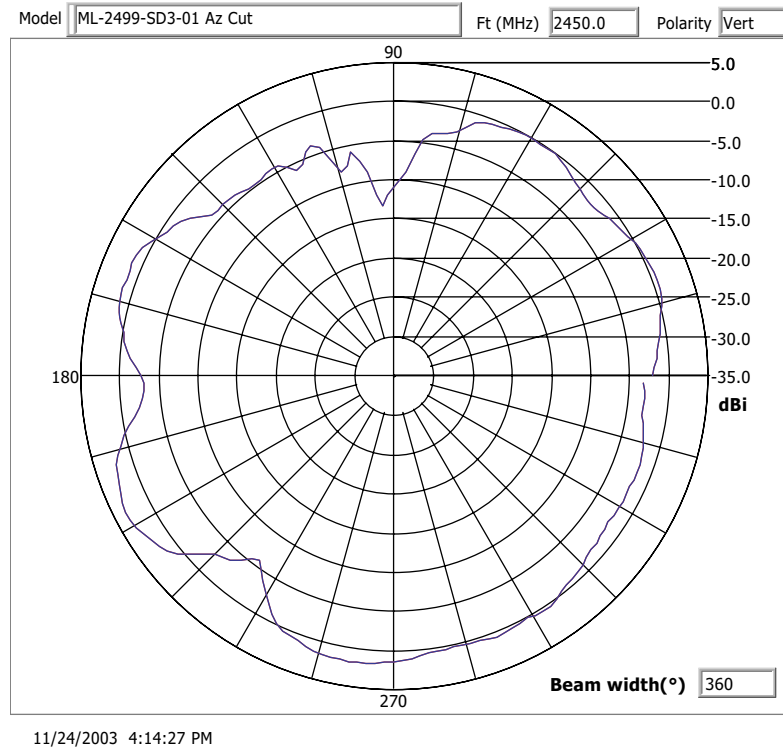
Azimuth Pattern
