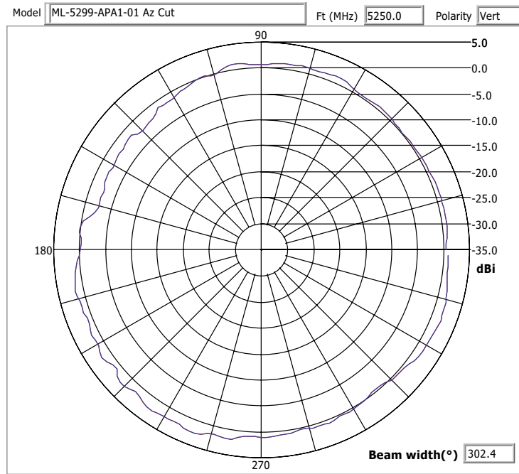
Azimuth Pattern
