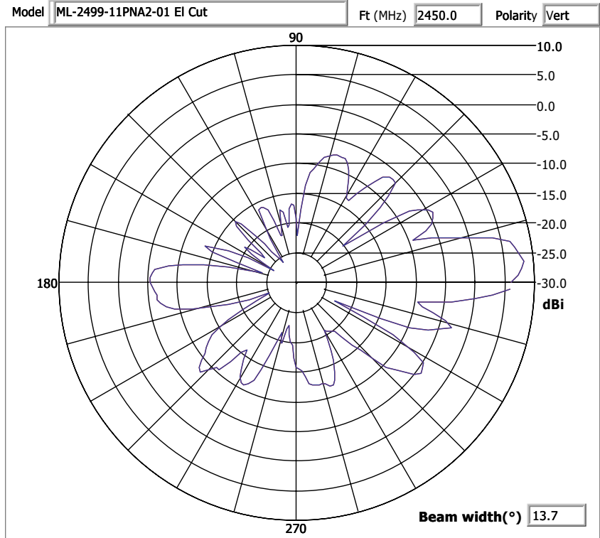
Elevation Pattern
