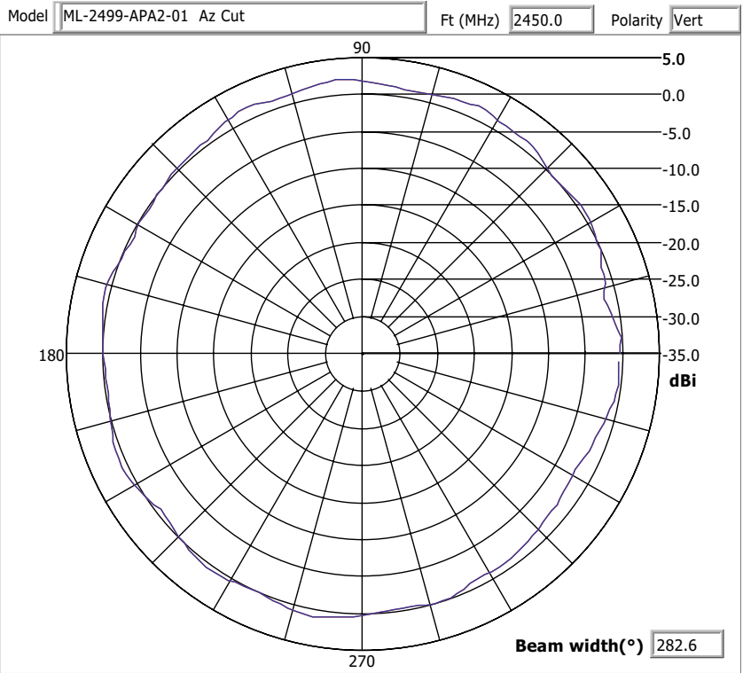
Azimuth Pattern
