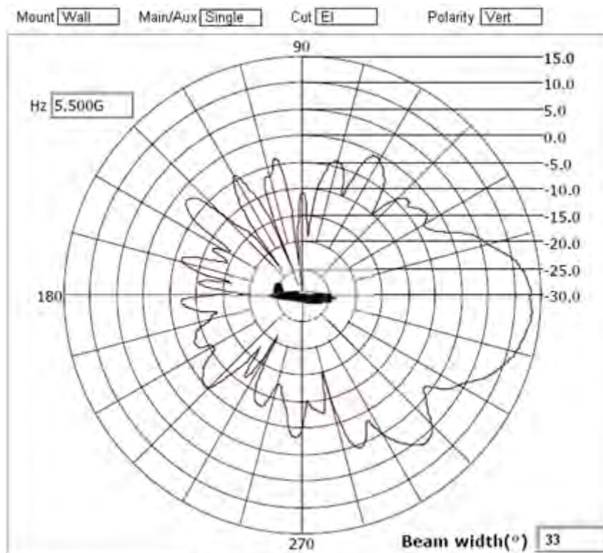
Elevation Pattern
