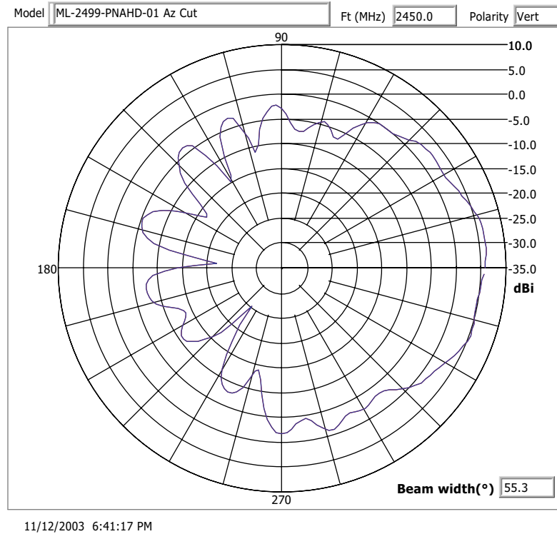
Azimuth Pattern
