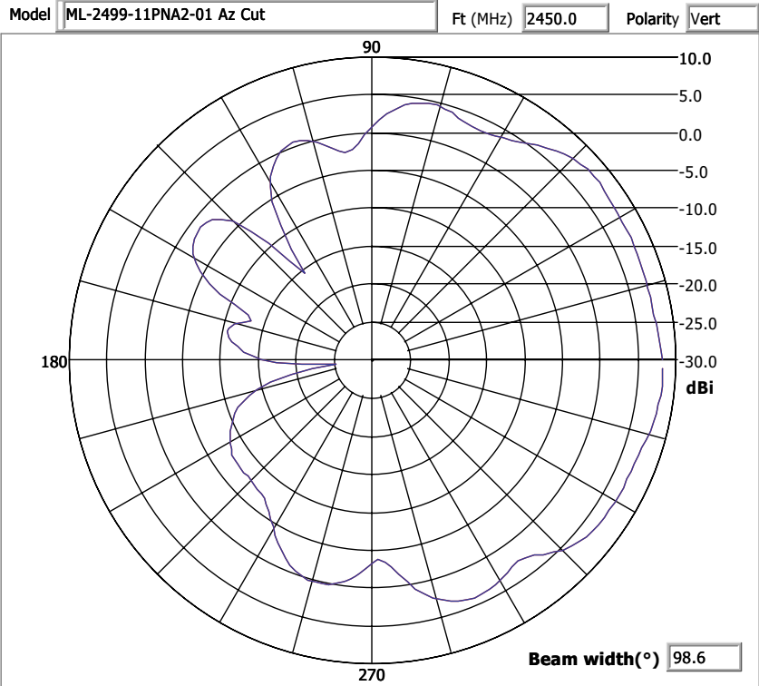
Azimuth Pattern
