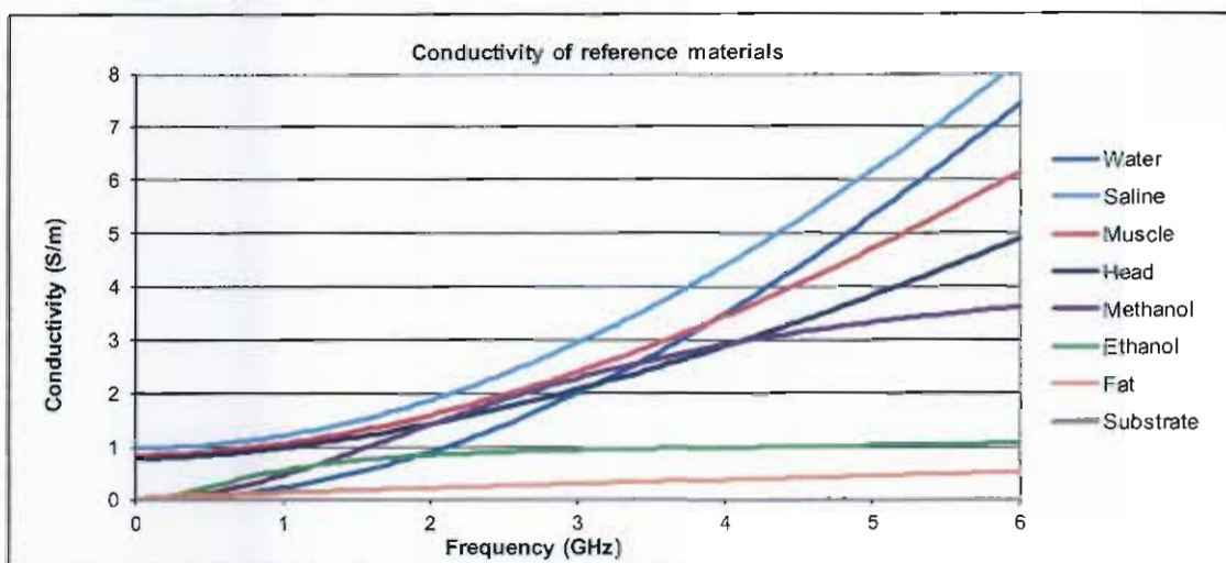
Fig. B.2 Conductivity of reference materials
