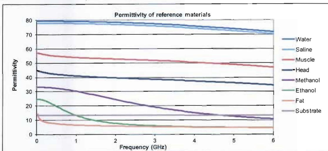
Fig. B.1 Permittivity of reference materials
