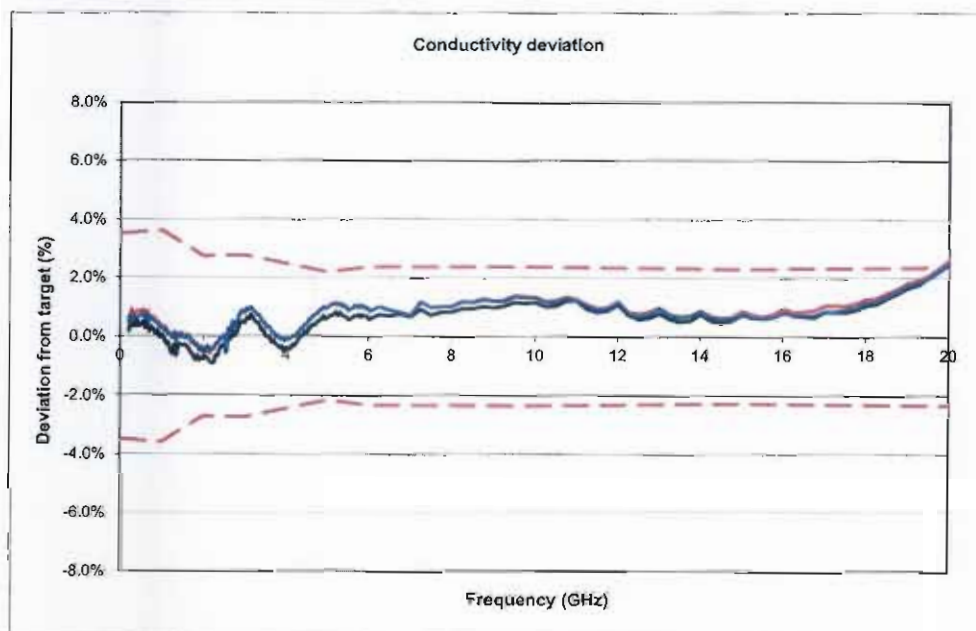
Fig. 4.2 HSL conductivity deviation from target, 200 MHz – 20 GHz
