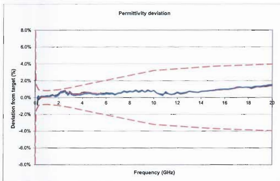
Fig. 3.1 Methanol permittivity deviation from target, 200 MHz – 20 GHz
