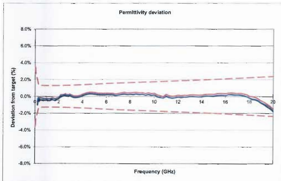
Fig. 4.1 HSL permittivity deviation from target, 200 MHz – 20 GHz
