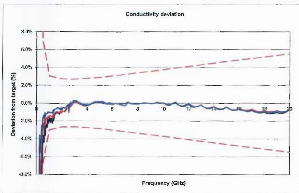
Fig. 3.2 Methanol conductivity deviation from target, 200 MHz – 20 GHz
