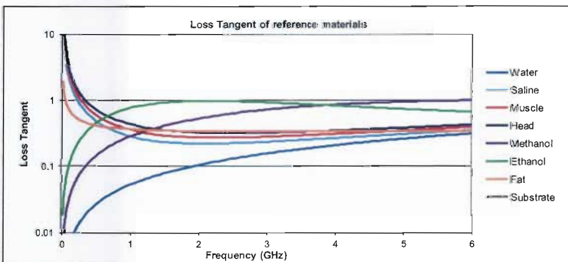
Fig. B.3 Loss tangent of reference materials
