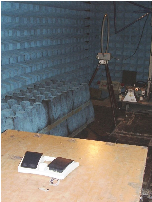
Investigation radiated emissions test of foot pedal transmitter with loop antenna.
