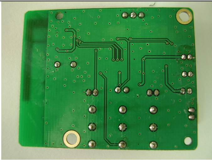
Pedal. PCB Rear view.
