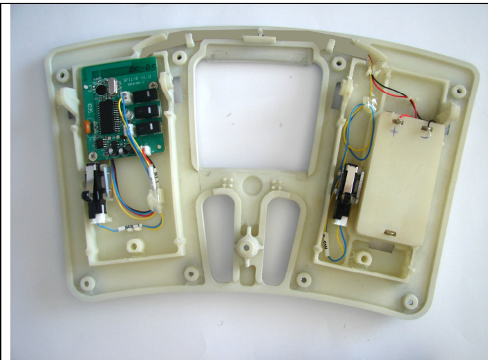
Pedal. Internal view.
