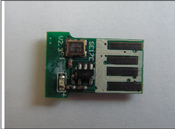
Dongle. PCB Upper view.
