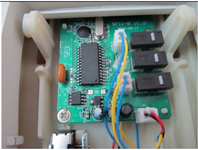
Pedal. PCB view.
