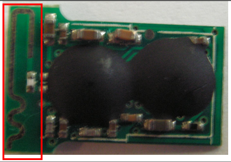
Dongle. PCB rear view with antenna.
