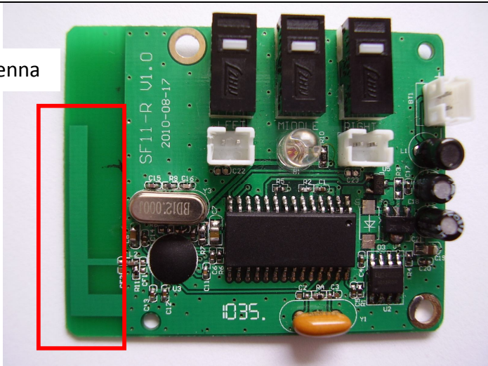
Pedal. PCB view with antenna.
