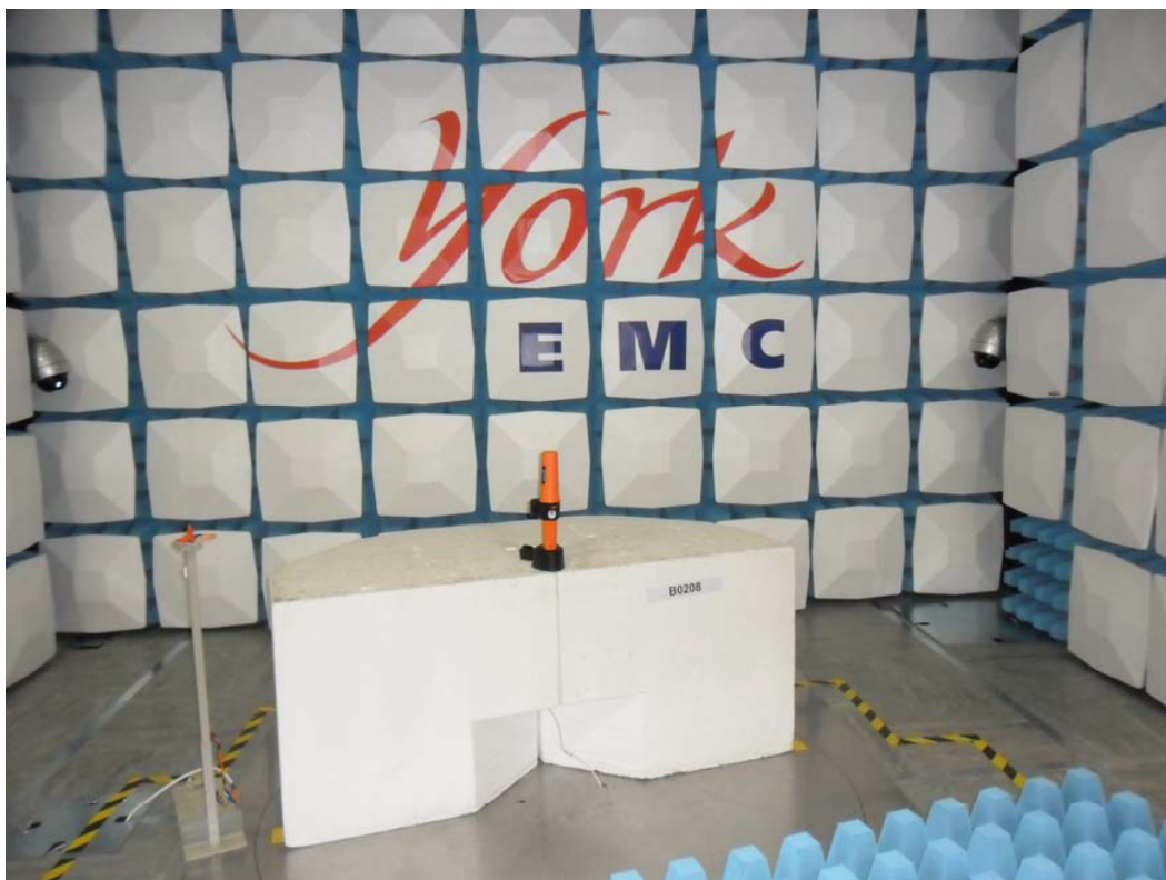
Figure 5.6.6 Radiated Immunity Testing
