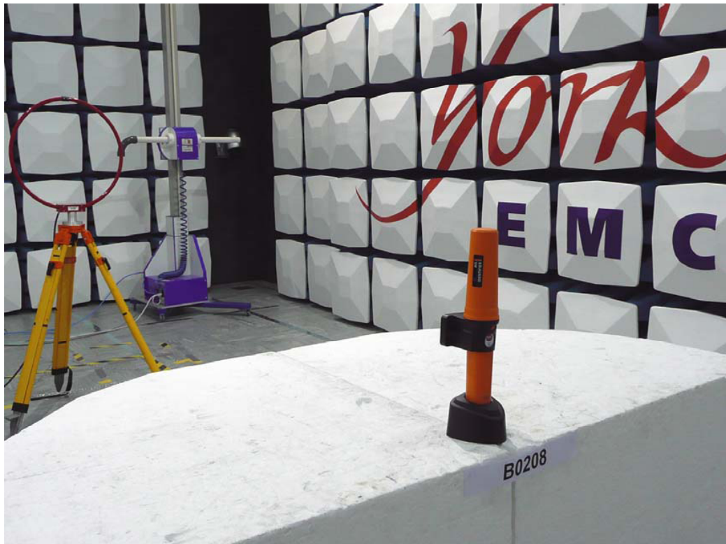
Figure 5.6.1 Radiated Emissions 0.15MHz to 30MHz Testing
