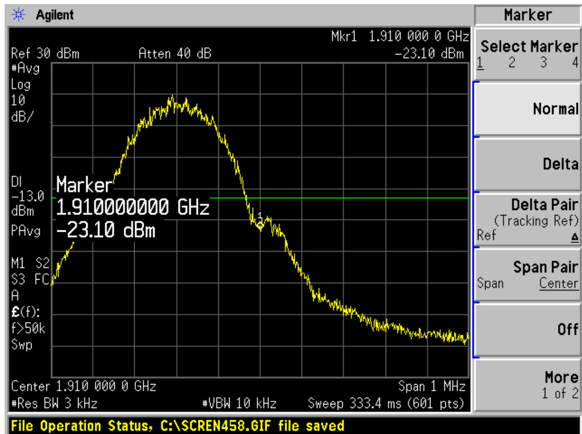
GSM1900+GPRS 810 Channel
