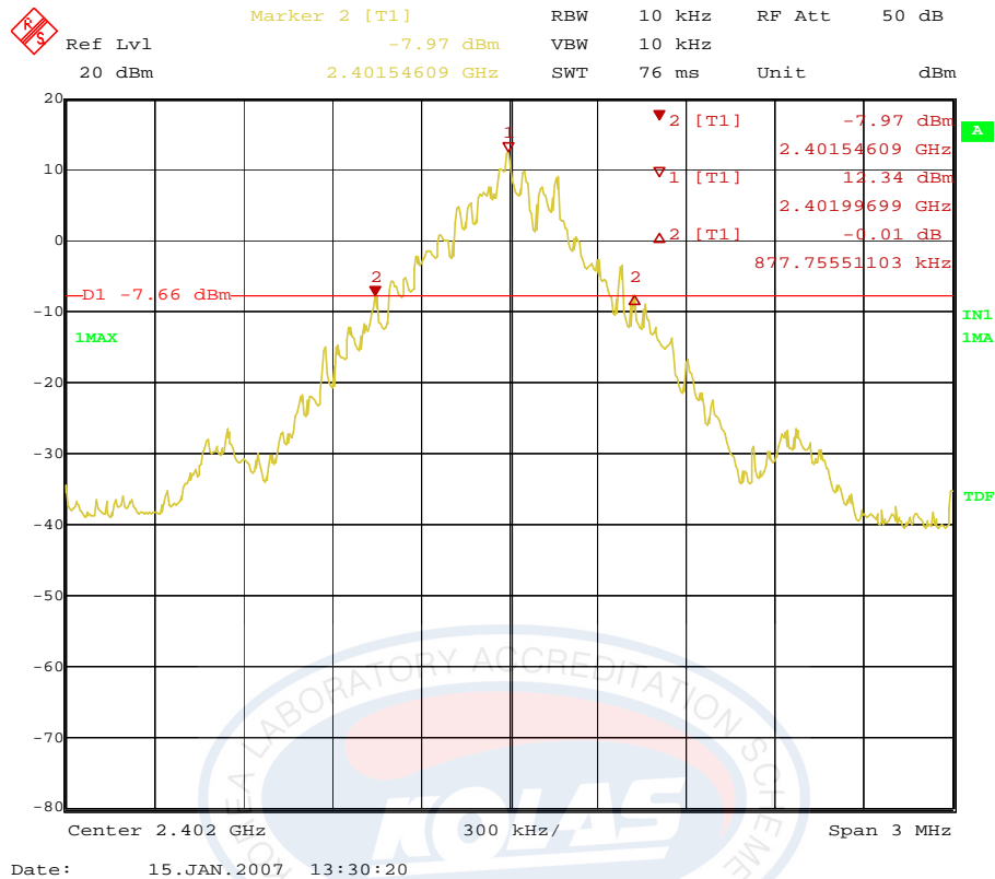
Figure 3. Plot of the 20dB Channel Bandwidth (Conducted)
