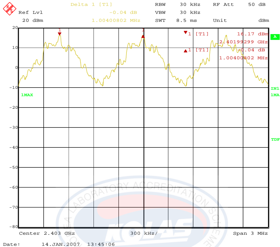
Figure 2. Plot of the Carrier Frequency Separation (Conducted)
