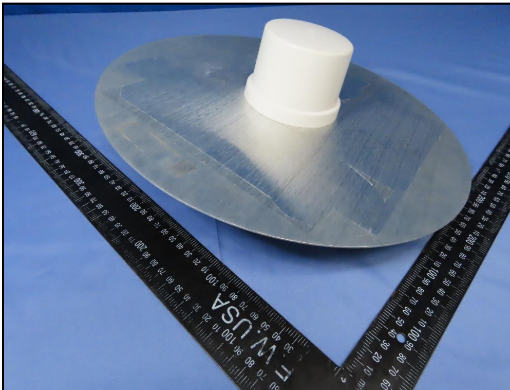
Antenna_WLAN 4 (Brand: Cradlepoint, Model: CP01)
