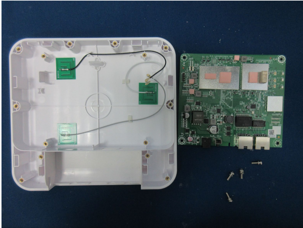
(6) EUT Photo / Ant. 1, Model No.: KG568-T4-175B17U7S (Internal Antenna)
