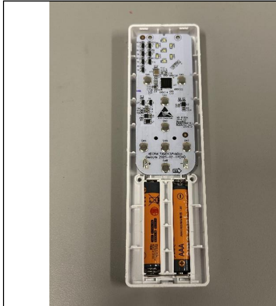
STANDALONE ON A TEST JIG (FRONT)
