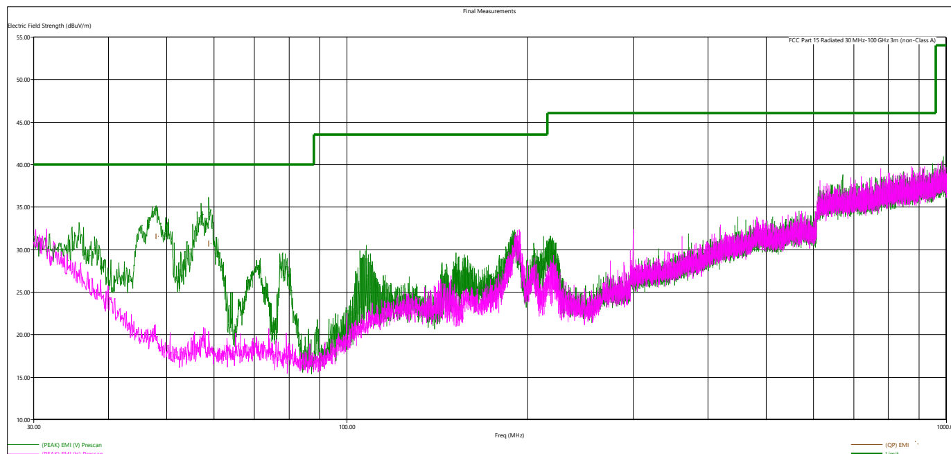
Figure 6 - Radiated Emissions Plot, Low Channel, BLE
