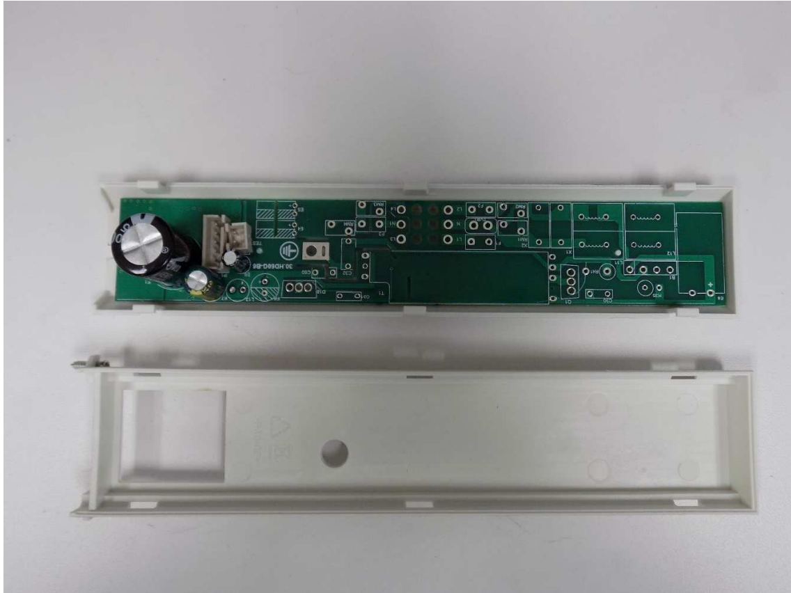
Figure 29: Housing PCBA 2
