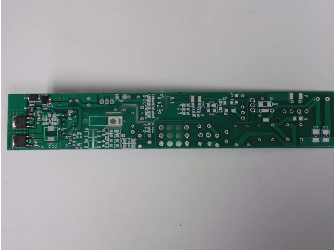
Figure 31: PCBA 2 Bottom
