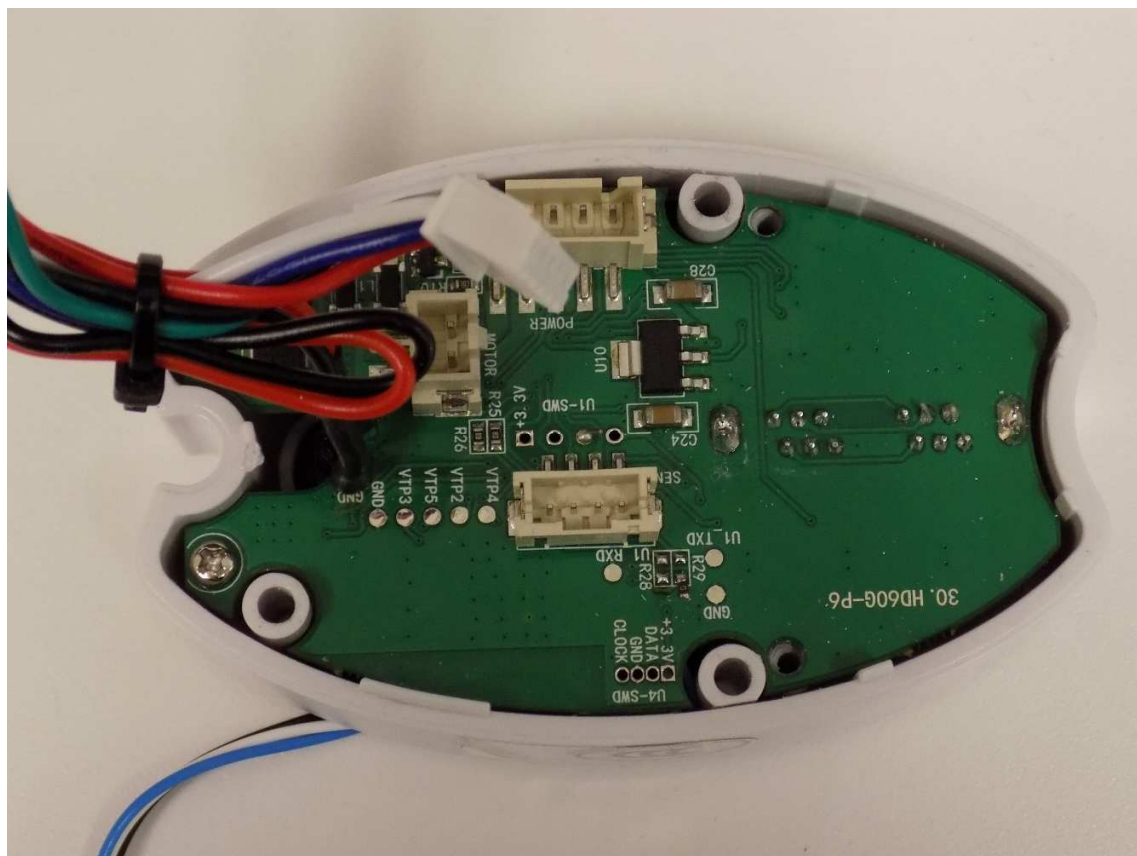
Figure 24: PCBA 1 Top (Housing)
