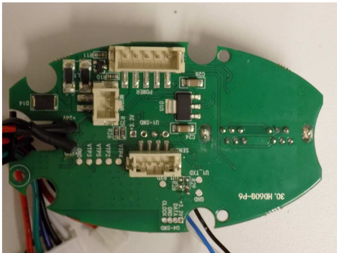
Figure 25: PCBA 1 Top
