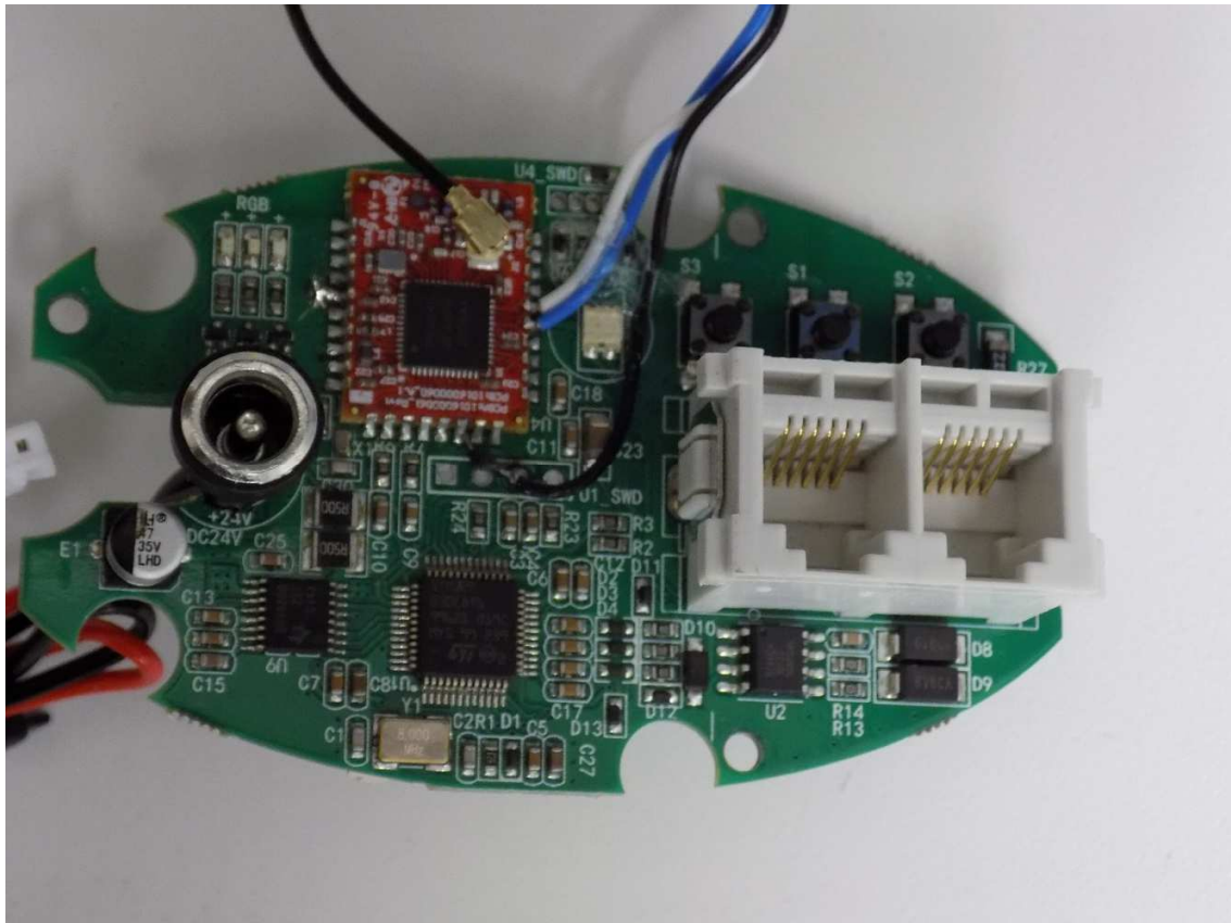
Figure 26: PCBA 1 Bottom
