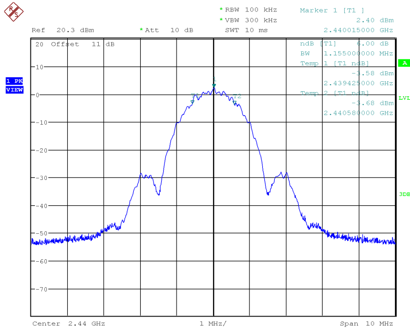
Plot 15. 2440MHz, 6dB Bandwidth, 2Mbps
