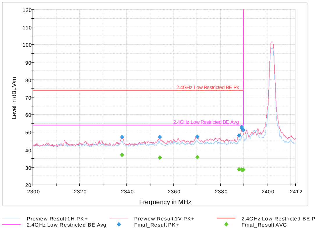
Plot 19. 2402 MHz, 1Mbps Lower Band Edge, Restricted
