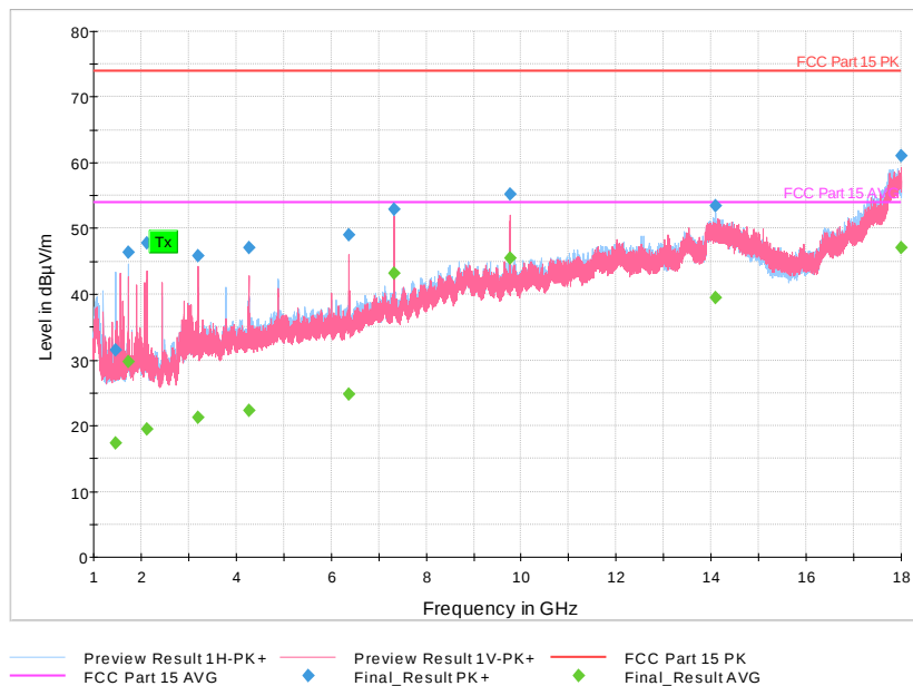
Plot 29. 1-18 GHz, 2440 MHz, 2Mbps
