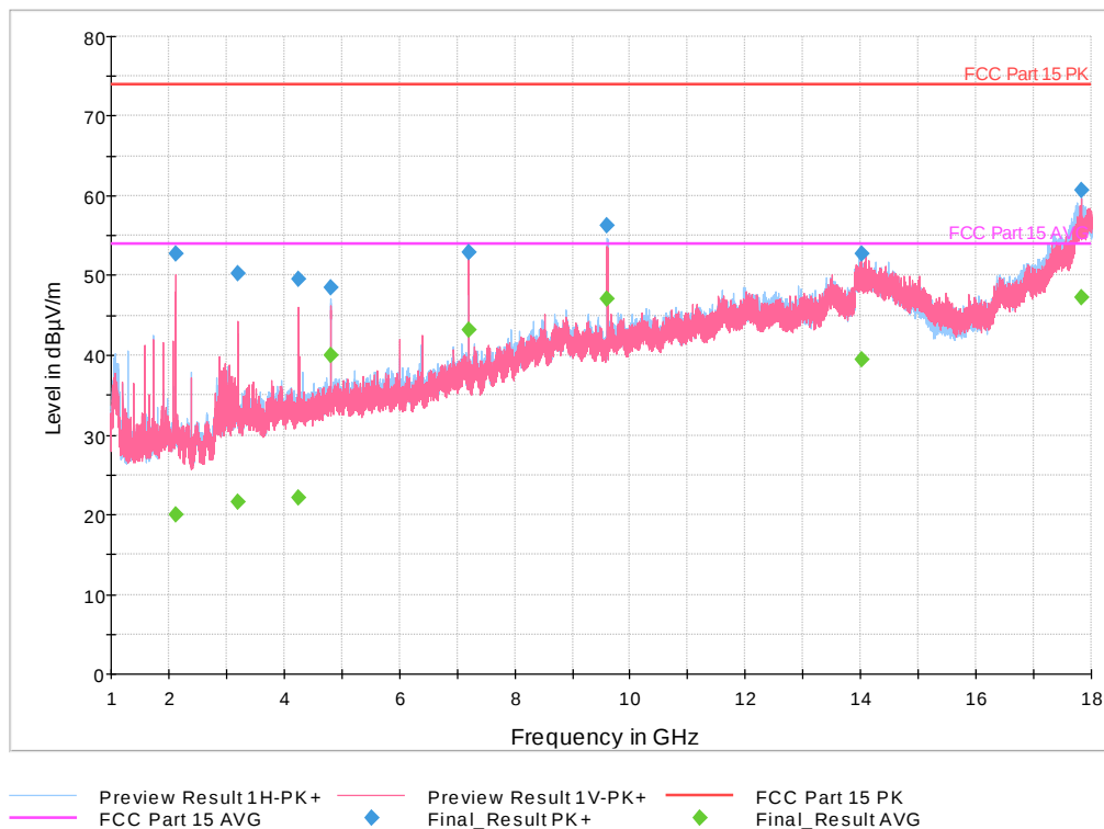
Plot 28. 1-18 GHz, 2402 MHz, 2Mbps
