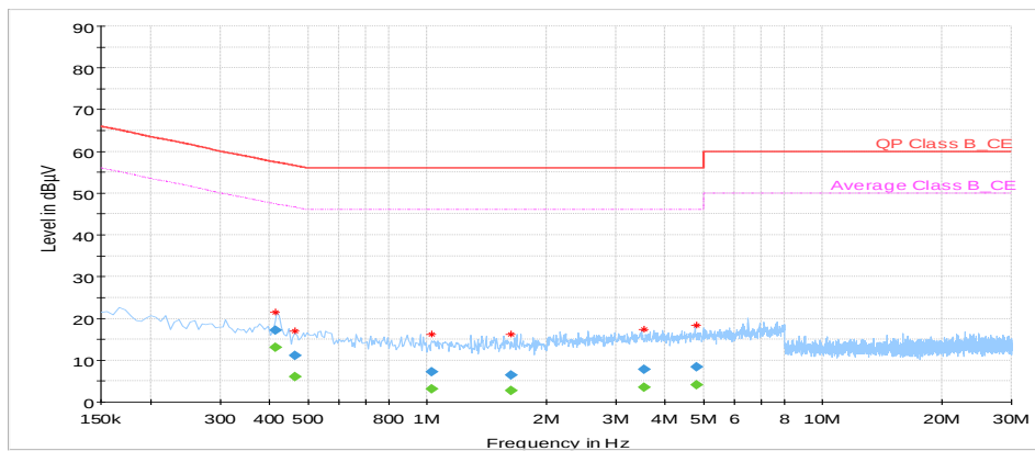
Plot 31. 0.15 - 30 MHz, Live Line
