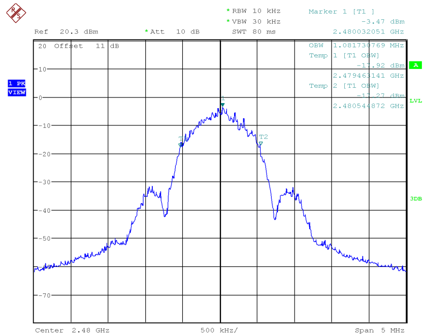
Plot 12. 2480MHz, 99% Bandwidth, 1Mbps
