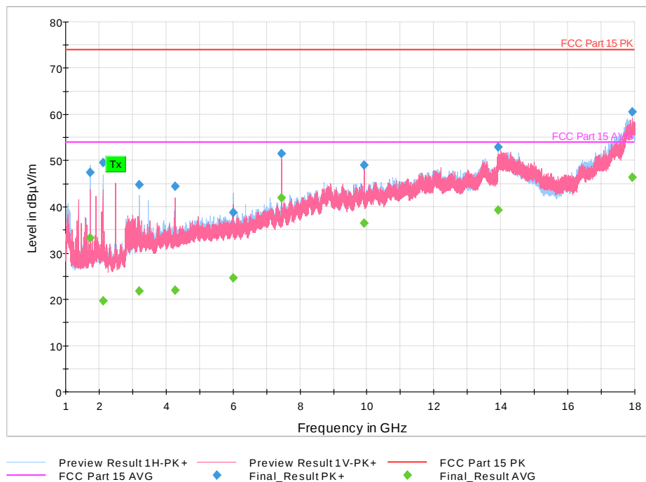
Plot 30. 1-18 GHz, 2480 MHz, 2Mbps
