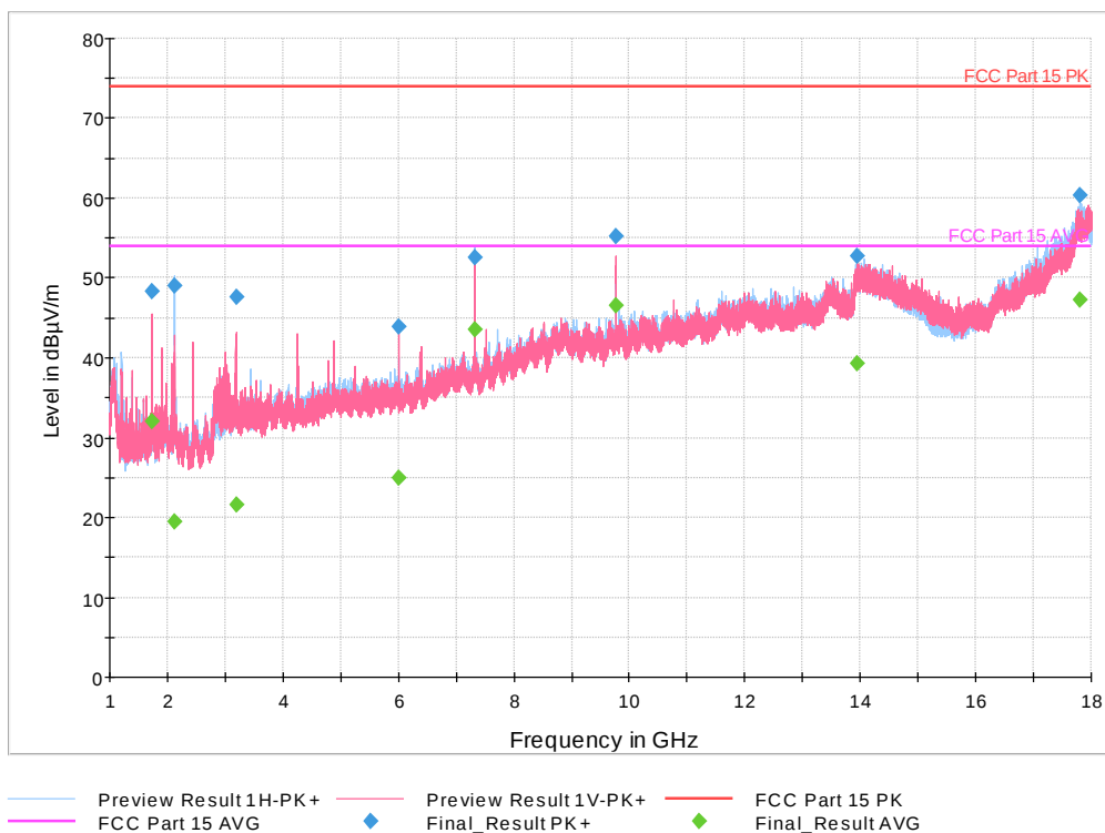
Plot 26. 1-18 GHz, 2440 MHz, 1Mbps
