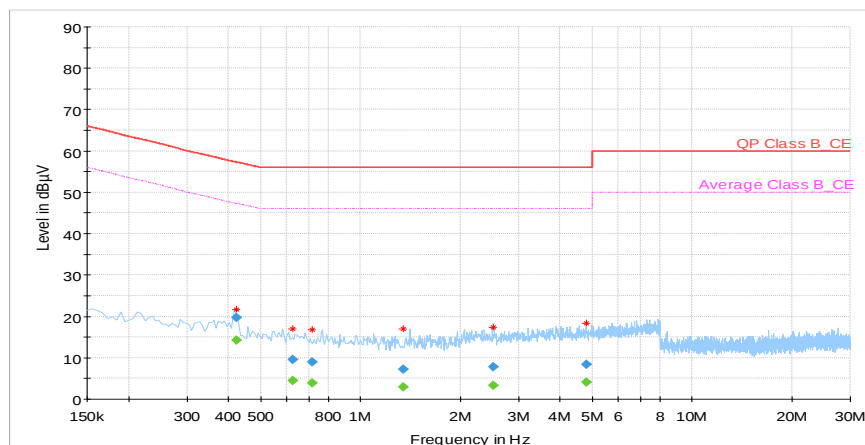
Plot 32. 0.15 - 30 MHz, Neutral Line
