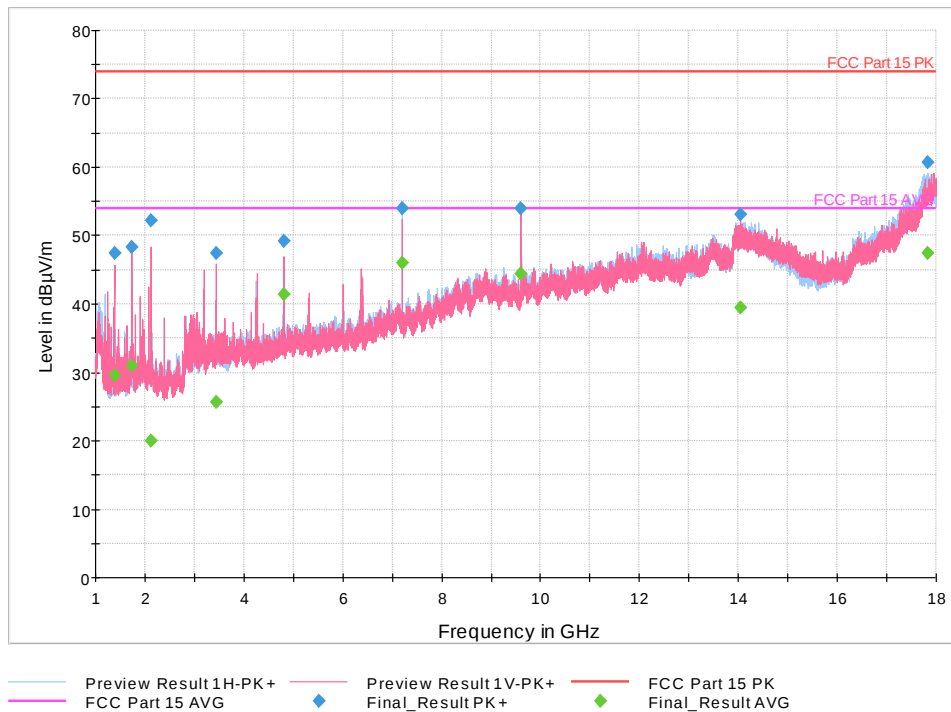
Plot 25. 1-18 GHz, 2402 MHz, 1Mbps
