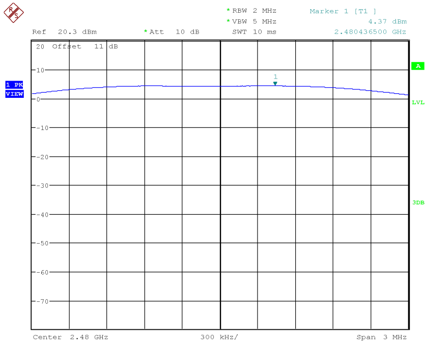
Plot 6. Maximum Conducted Power, 2480MHz, 2Mbps
