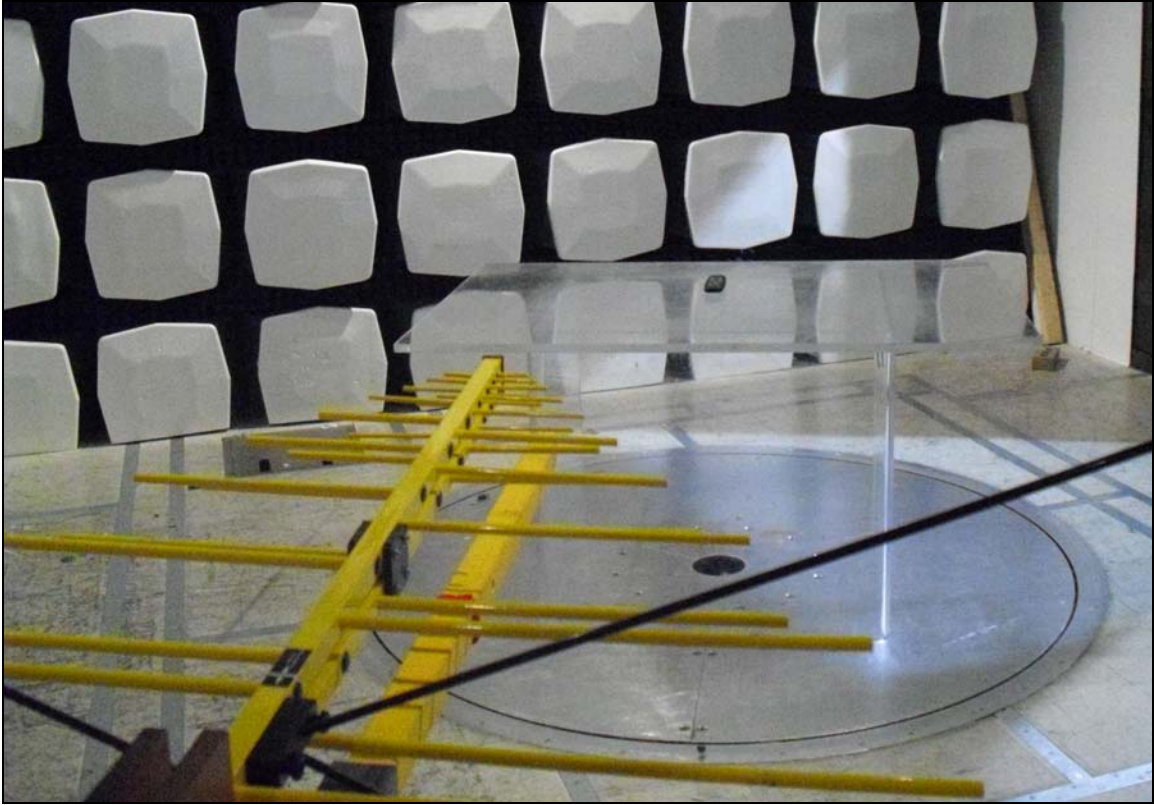
Photograph 1. Radiated Emissions
