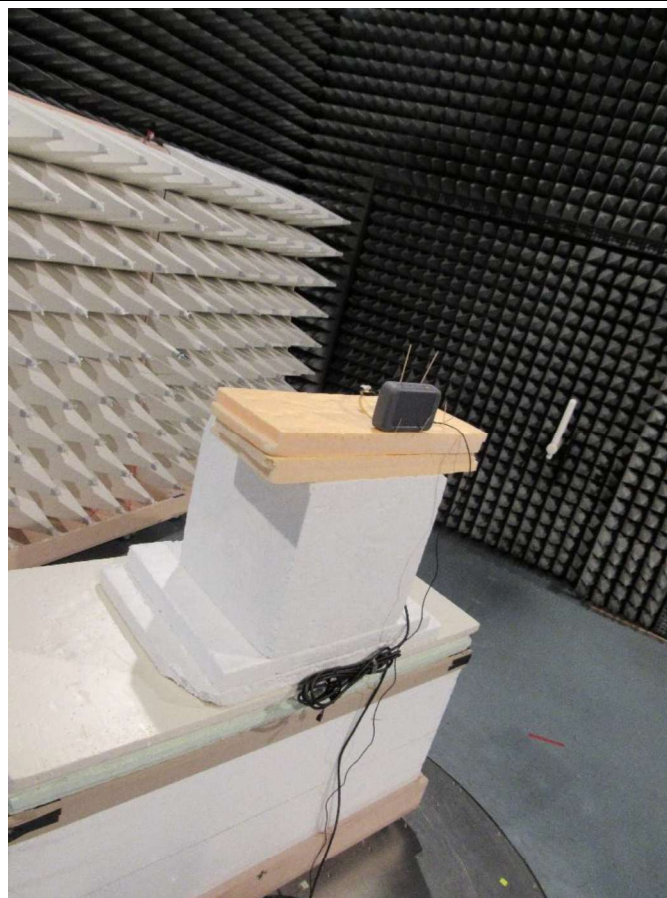
Test setup above 1GHz - C
