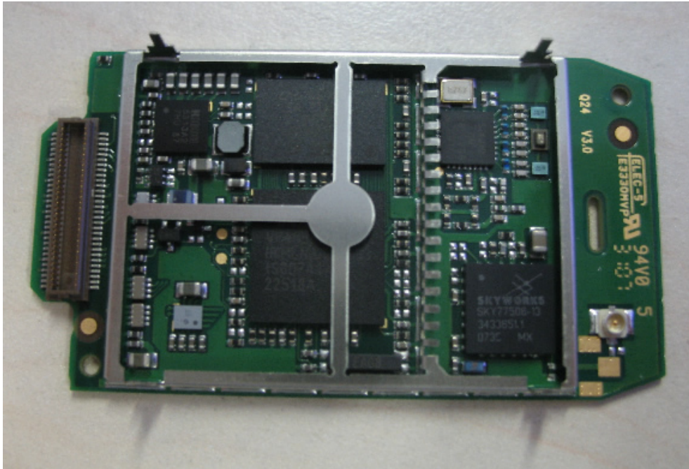
RADIO MODULE INTERNAL WIEV (Without protection shield)
