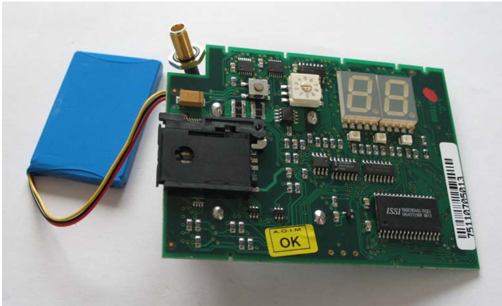
GSM Board with modem (Side 1)
