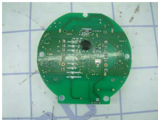
PCB Solder
