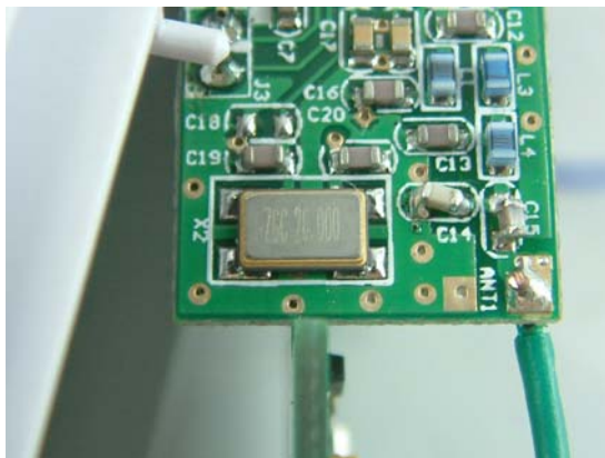
RZ250W Oscillation view 1
