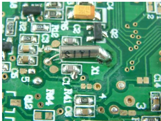
Z270W Oscillation view 2
