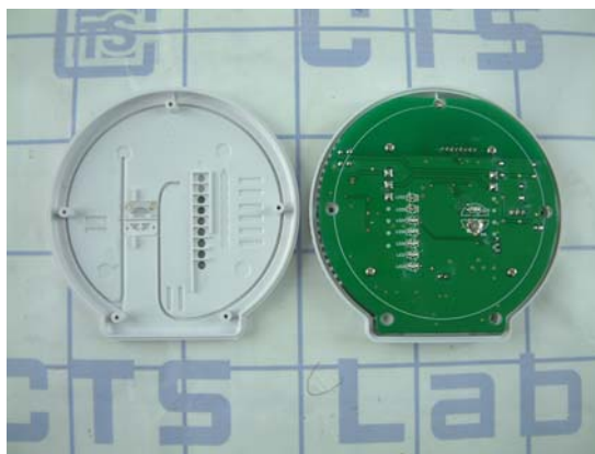
Z260W Internal view
