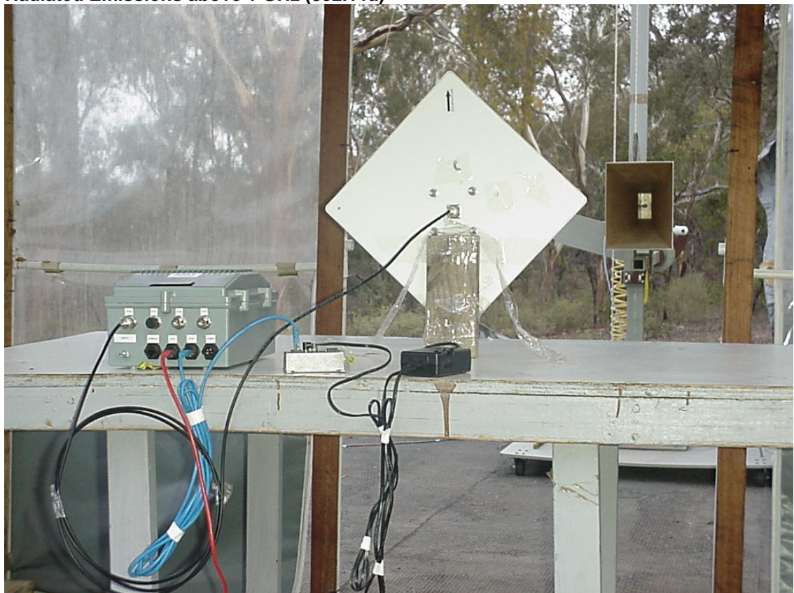
Radiated Emissions above 1 GHz (802.11a)
