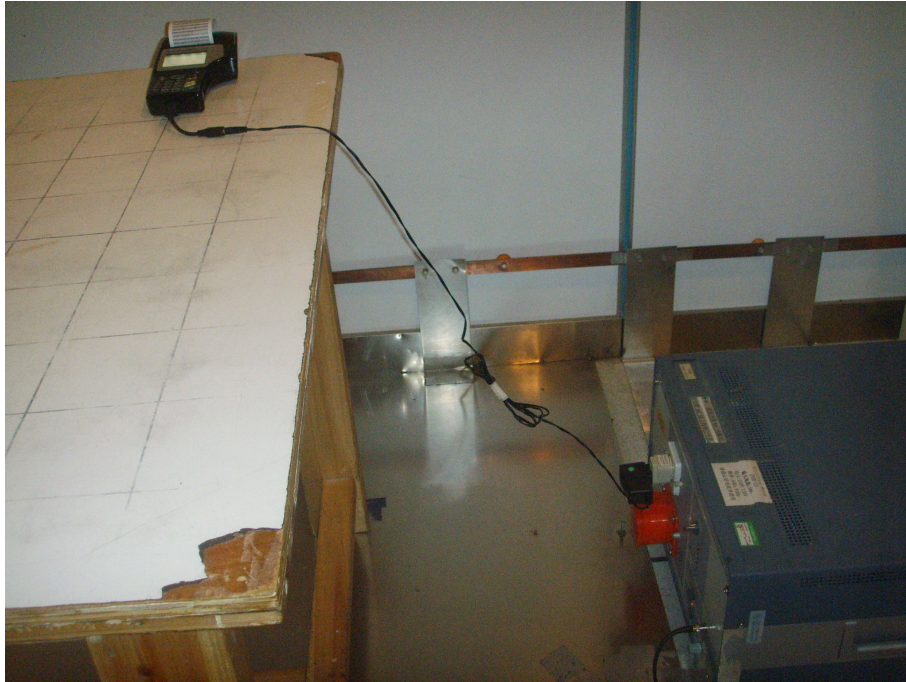
Conduction Emission Test – Front View
