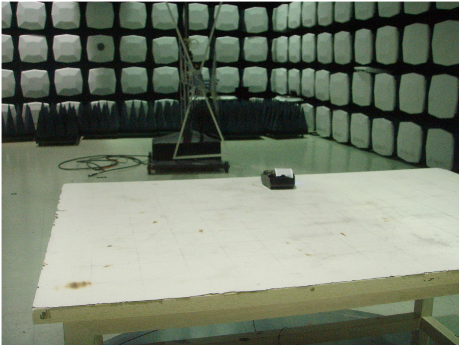
Radiation Emission Test – Rear View
