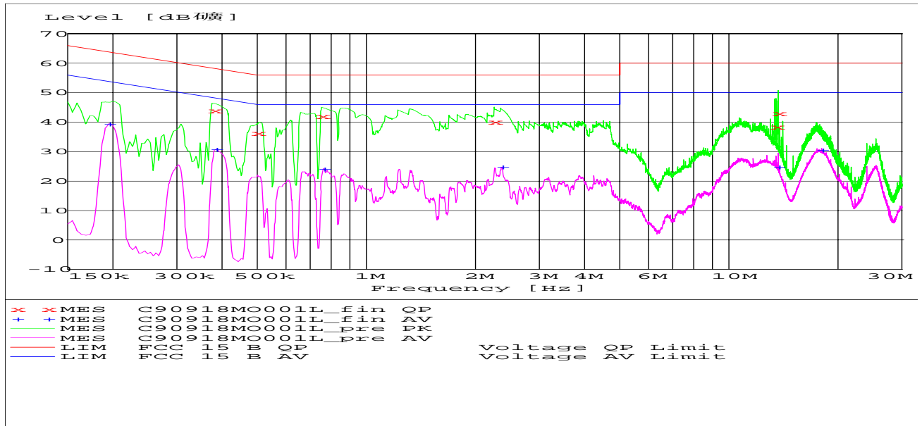
(Plot:L Phase)
