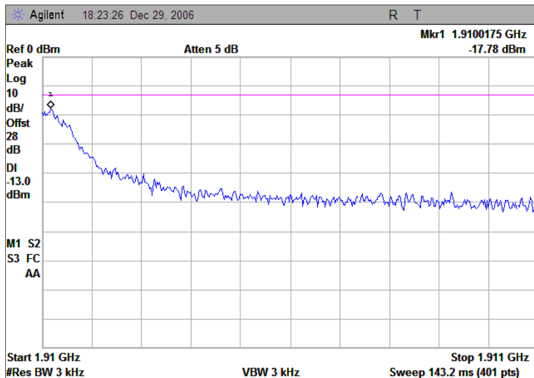
(Plot B: Channel = 810)
