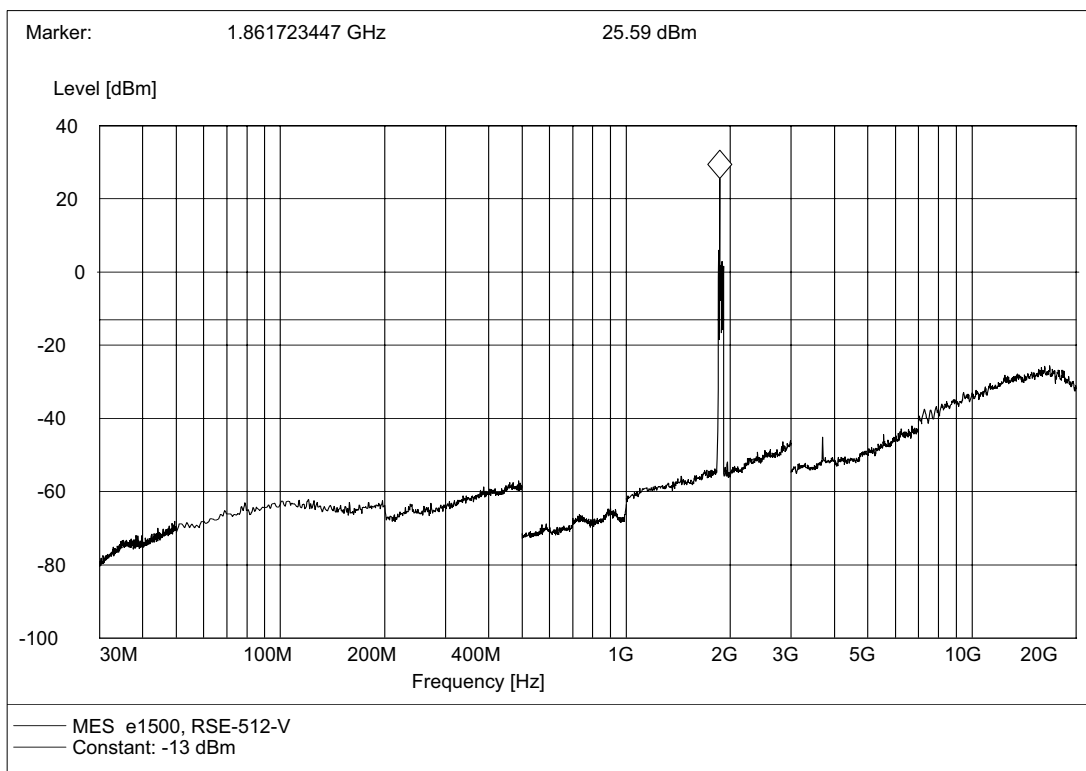
(Plot A.2: Channel = 512, Test Antenna Vertical)
