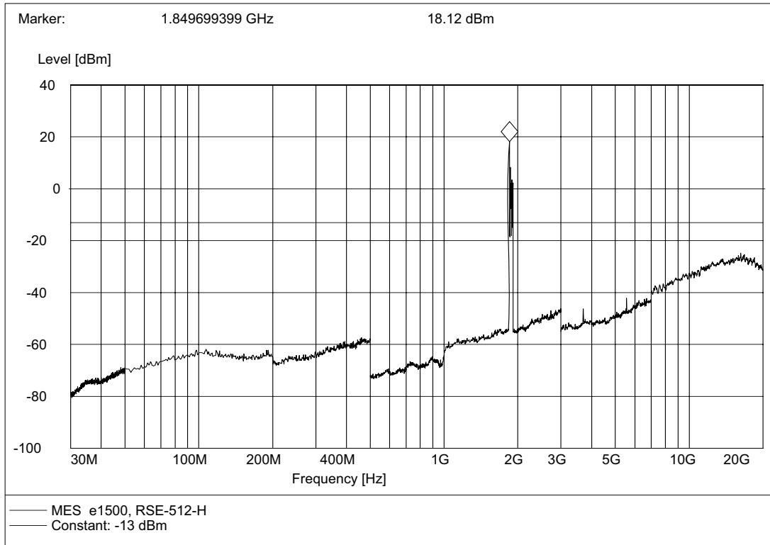
(Plot A.1: Channel = 512, Test Antenna Horizontal)
