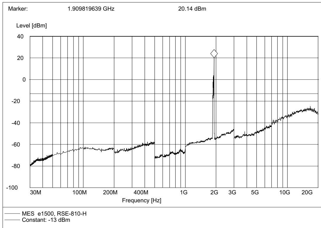
(Plot C.1: Channel = 810, Test Antenna Horizontal)
