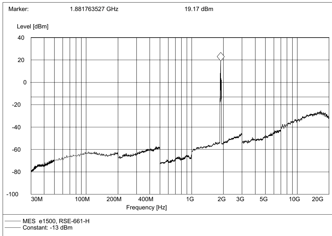
(Plot B.1: Channel = 661, Test Antenna Horizontal)
