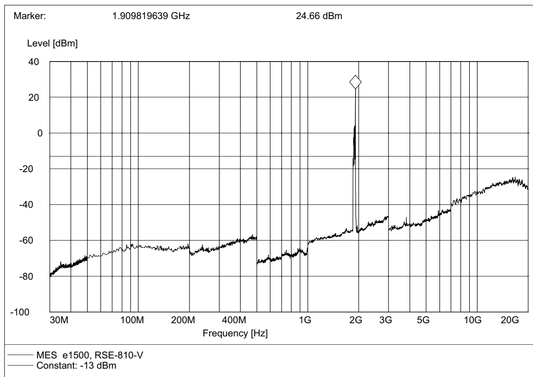
(Plot C.2: Channel = 810, Test Antenna Vertical)
