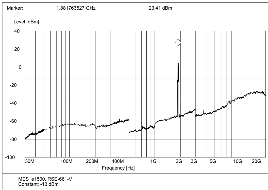
(Plot B.2: Channel = 661, Test Antenna Vertical)
